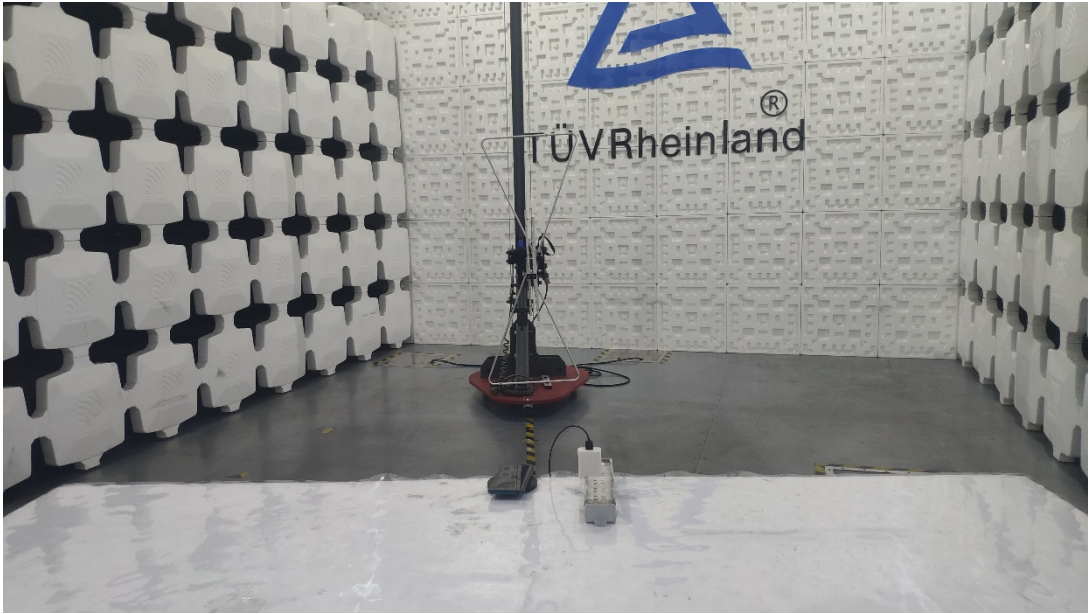
Photograph 4: Set-up for Radiated Emissions, below 1GHz
