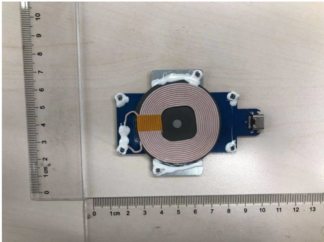
Fig. 4 Bottom view of mainboard (for all models)
