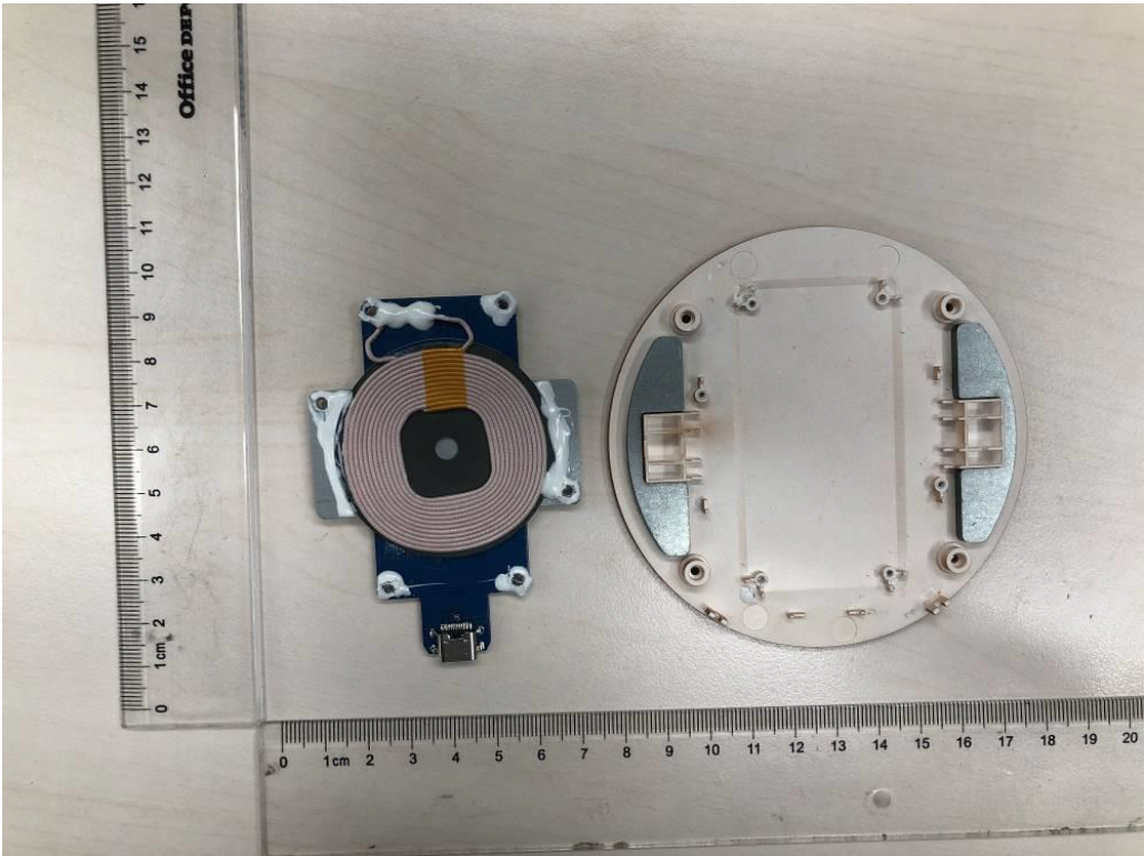
Fig 2 Internal view (for all models)
