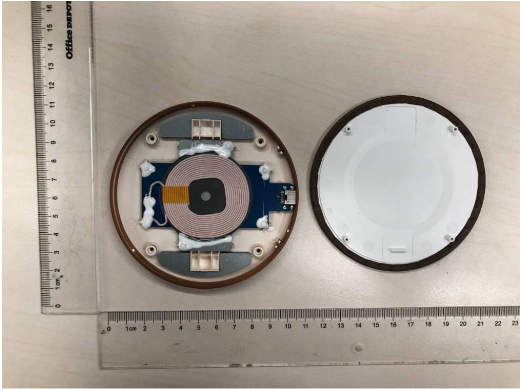
Fig. 1 Internal view (for all models)
