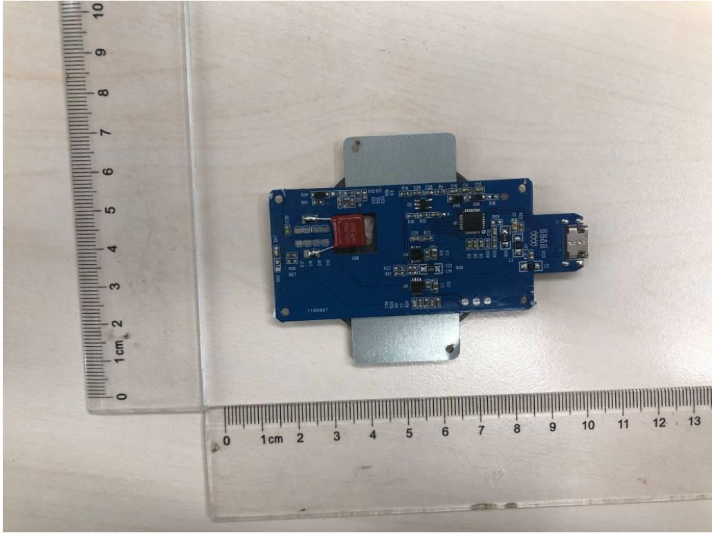
Fig. 3 Top view of mainboard (for all models)
