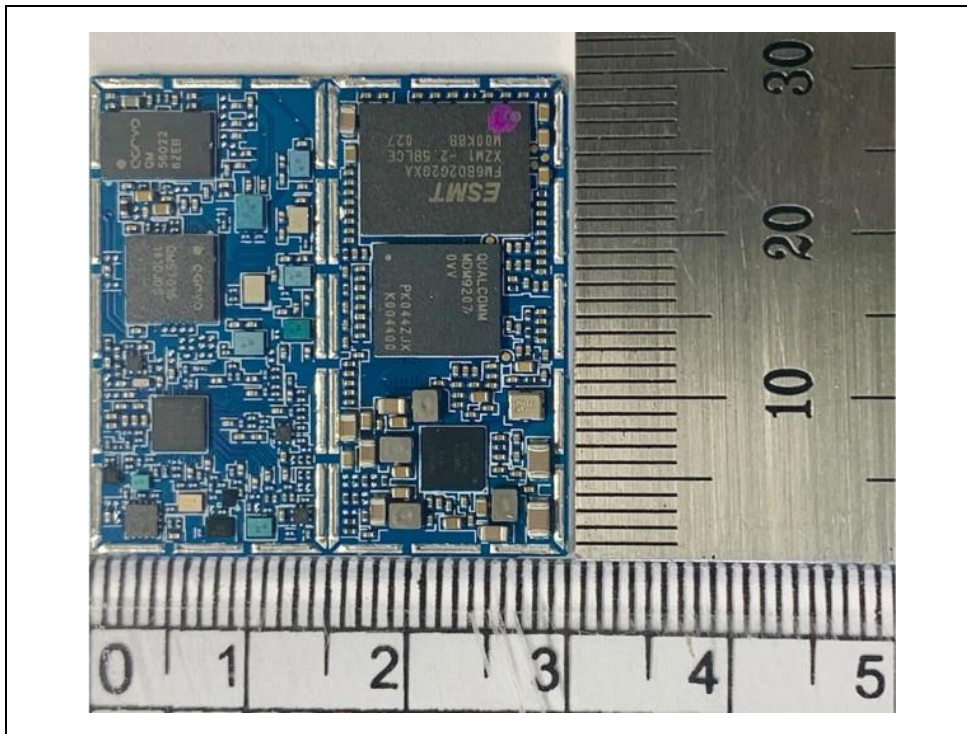
EUT Shield Can open (AML550)
