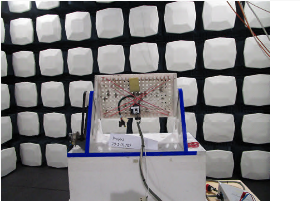
Photograph 3: EUT test setup in the fully anechoic chamber, close up view
