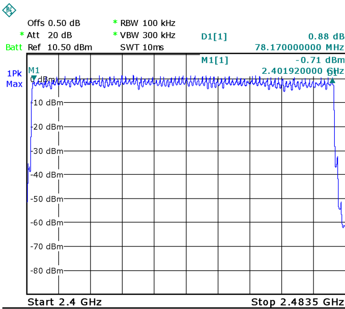
Modulation: 8DPSK
