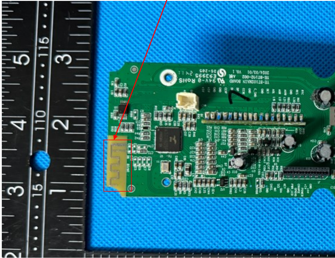
BT antenna
