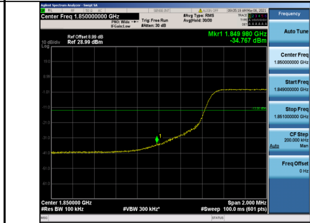
Band2-10MHz-16QAM-18650-50RB#0
