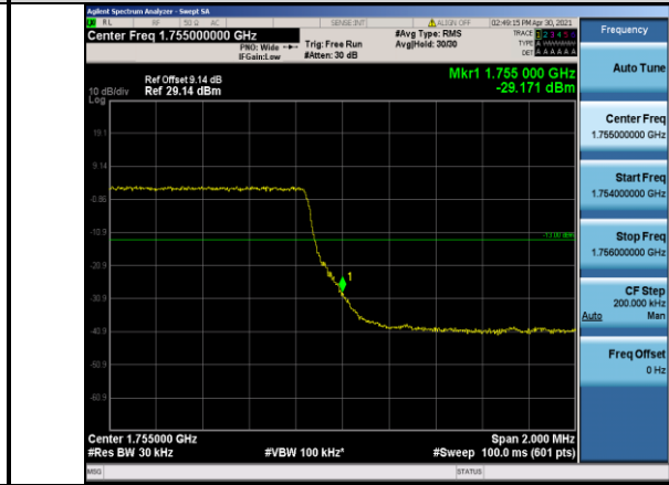
Band4-3MHz-QPSK-20385-15RB#0
