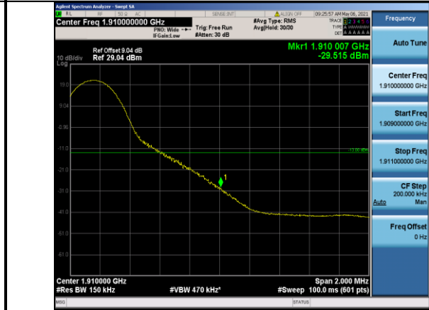
Band2-15MHz-QPSK-19125-1RB#74
