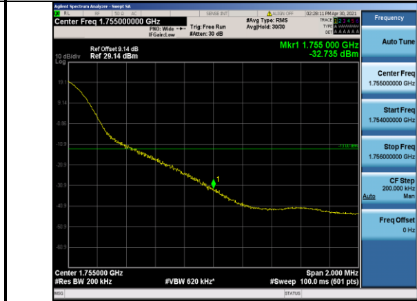
Band4-20MHz-16QAM-20300-1RB#99
