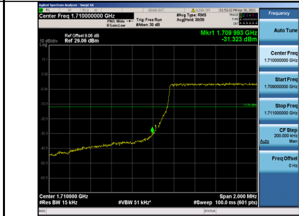
Band4-1.4MHz-16QAM-19957-6RB#0
