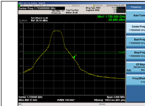
Band4-5MHz-QPSK-20375-1RB#24
