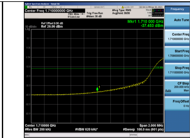
Band4-20MHz-16QAM-20050-100RB#0
