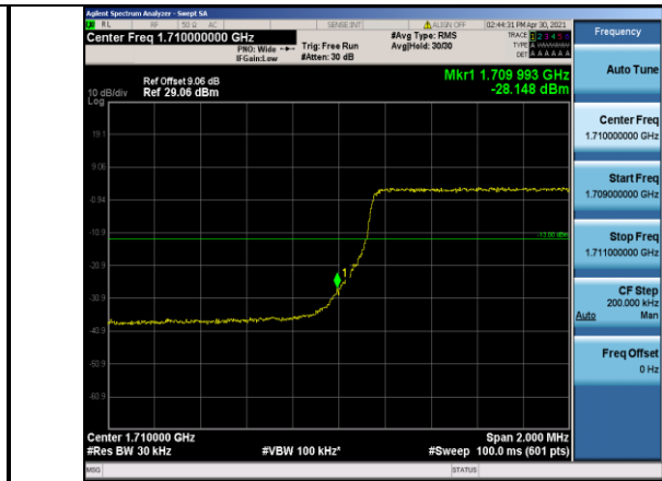
Band4-3MHz-QPSK-19965-15RB#0
