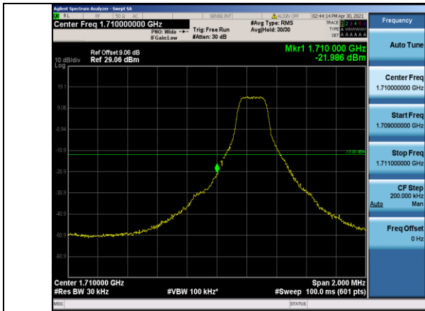
Band4-3MHz-16QAM-19965-1RB#0
