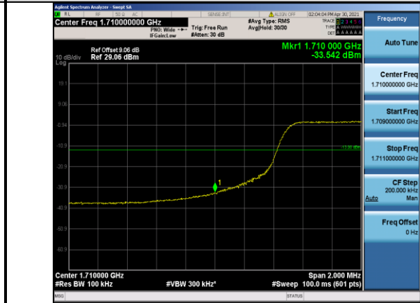
Band4-10MHz-16QAM-20000-50RB#0
