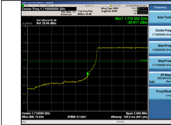
Band4-1.4MHz-QPSK-19957-6RB#0
