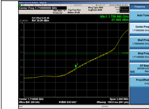
Band4-20MHz-16QAM-20050-1RB#0
