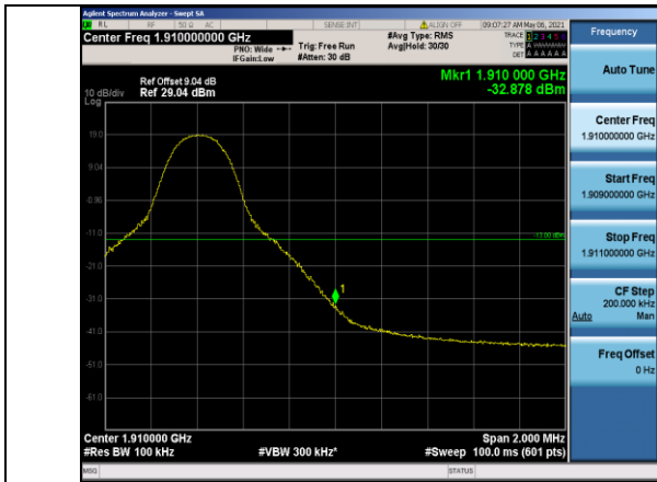
Band2-10MHz-16QAM-19150-1RB#49
