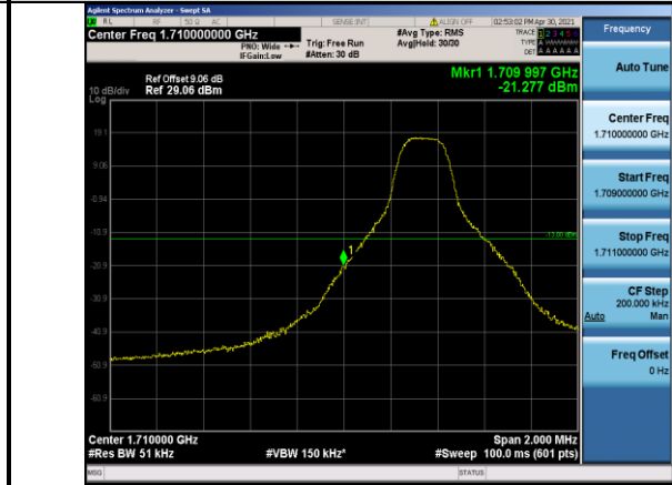
Band4-5MHz-QPSK-19975-1RB#0
