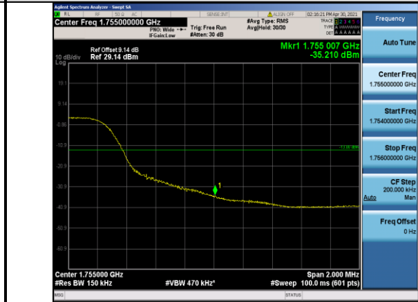
Band4-15MHz-QPSK-20325-75RB#0
