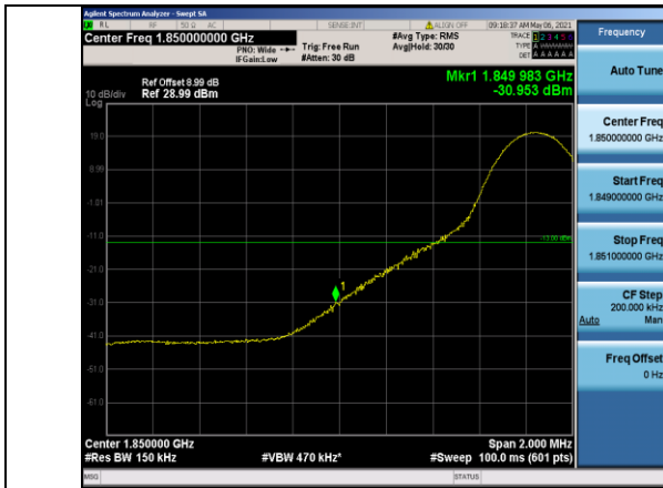
Band2-15MHz-16QAM-18675-1RB#0
