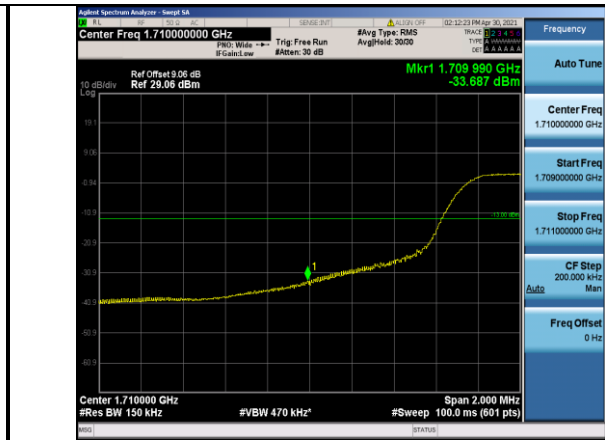
Band4-15MHz-QPSK-20025-75RB#0
