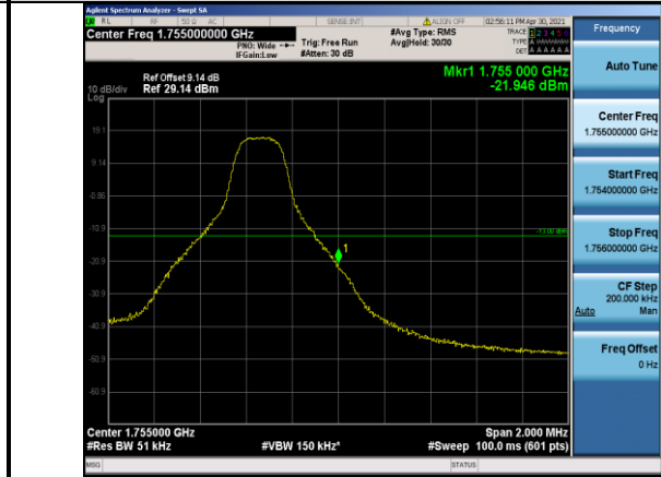
Band4-5MHz-16QAM-20375-1RB#24
