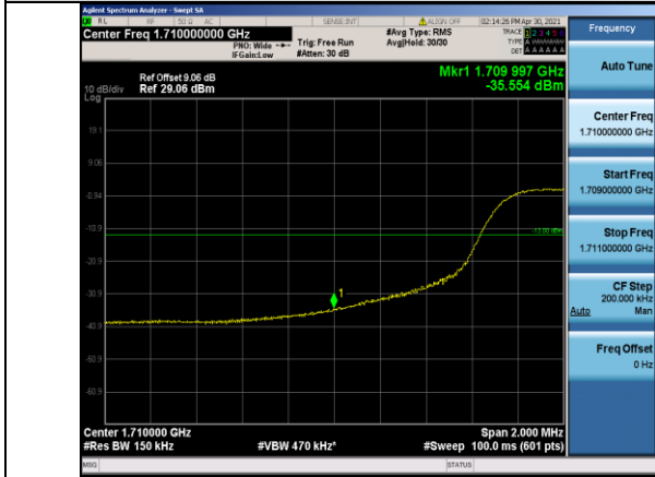
Band4-15MHz-16QAM-20025-75RB#0
