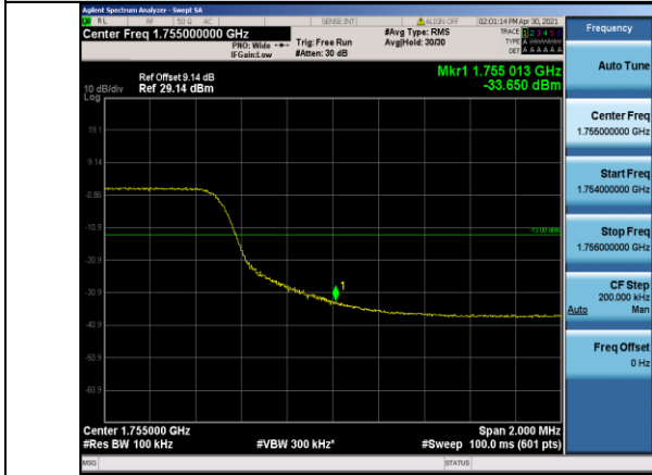
Band4-10MHz-16QAM-20350-50RB#0
