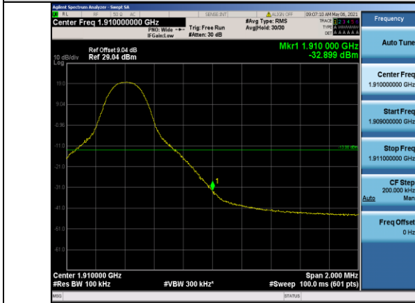
Band2-10MHz-QPSK-19150-1RB#49
