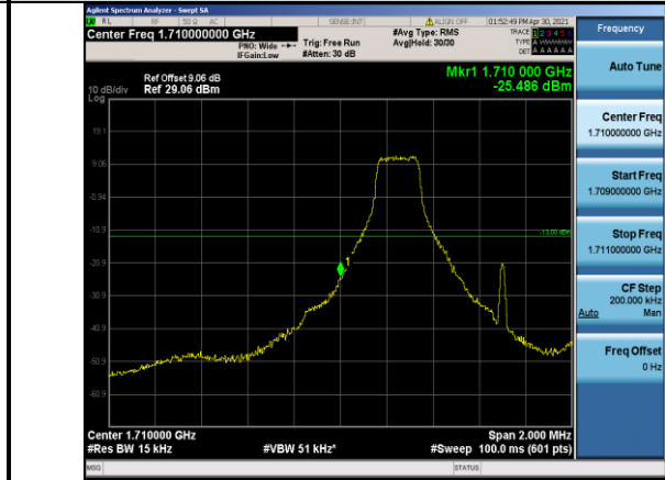
Band4-1.4MHz-16QAM-19957-1RB#0
