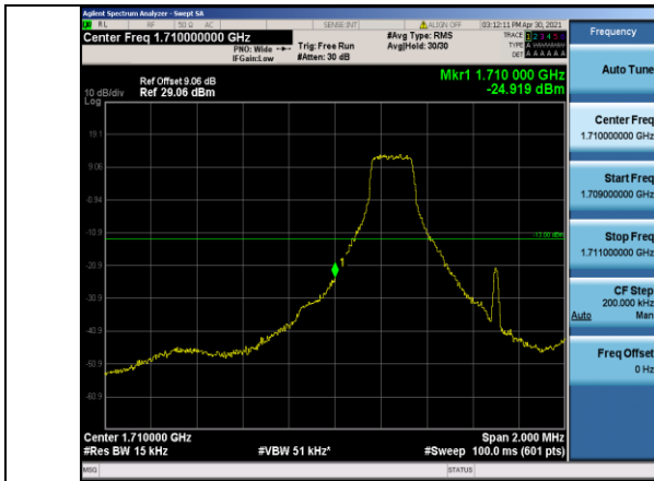
Band66-1.4MHz-QPSK-131979-1RB#0
