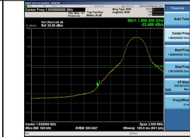
Band2-10MHz-16QAM-18650-1RB#0
