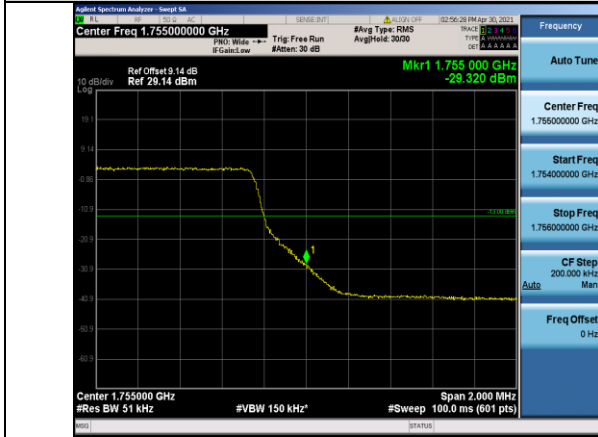
Band4-5MHz-QPSK-20375-25RB#0
