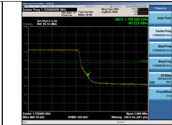
Band4-3MHz-16QAM-20385-15RB#0
