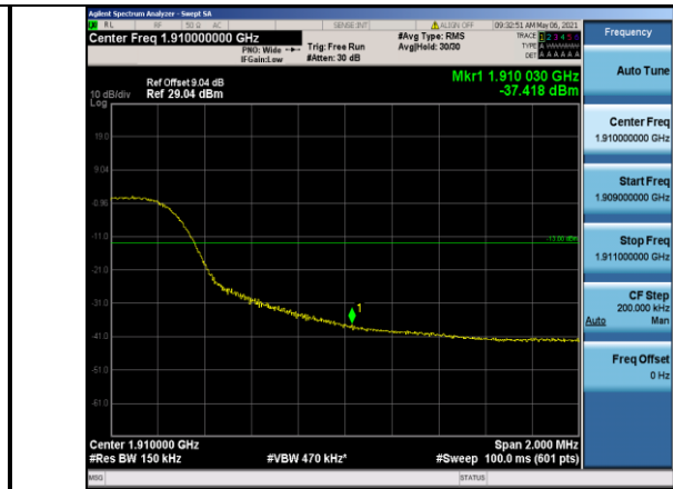
Band2-15MHz-16QAM-19125-75RB#0
