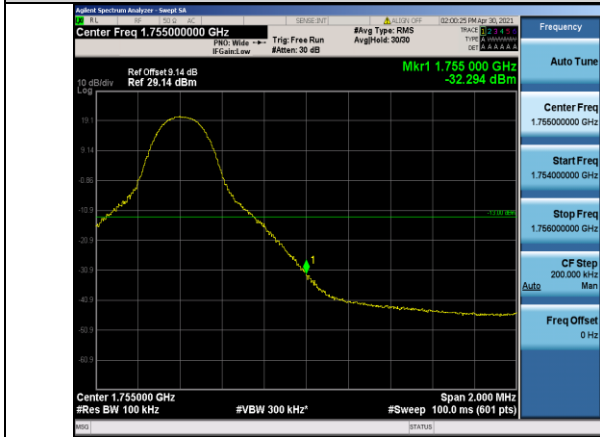
Band4-10MHz-QPSK-20350-1RB#49
