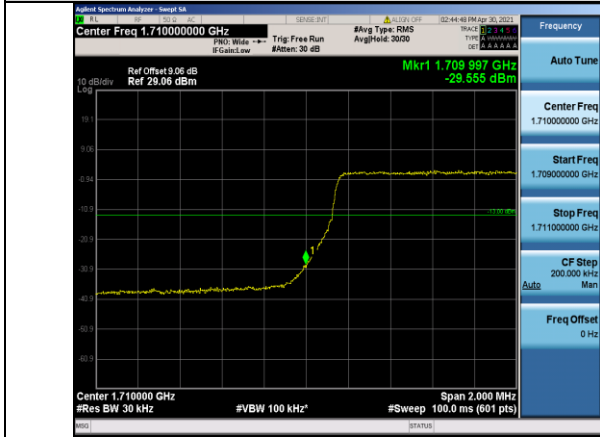
Band4-3MHz-16QAM-19965-15RB#0
