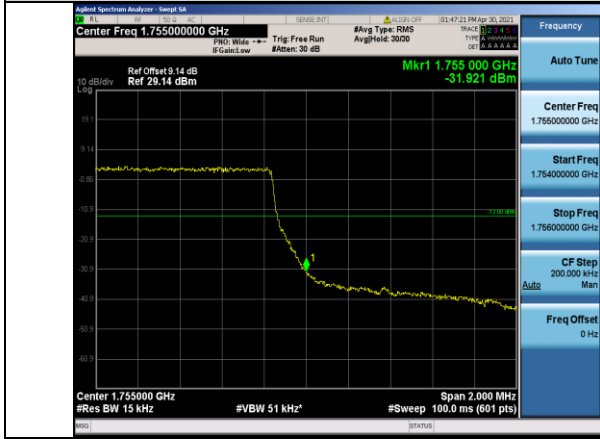
Band4-1.4MHz-16QAM-20393-6RB#0
