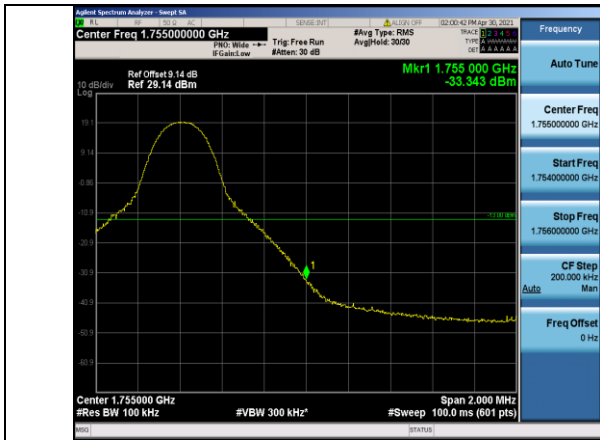
Band4-10MHz-16QAM-20350-1RB#49
