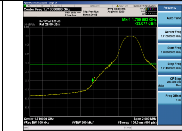
Band4-10MHz-16QAM-20000-1RB#0
