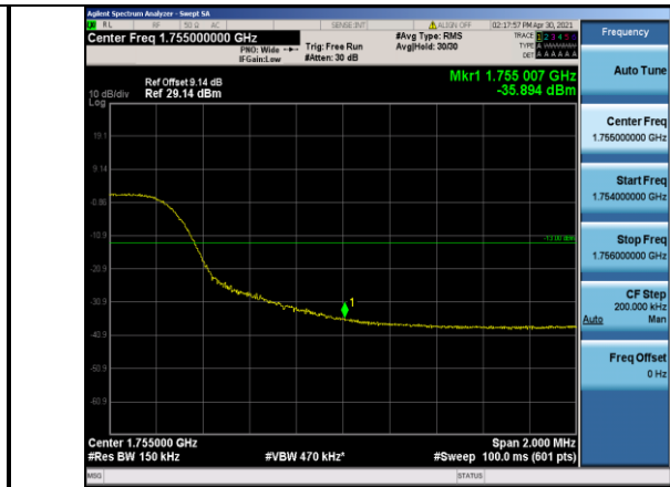
Band4-15MHz-16QAM-20325-75RB#0
