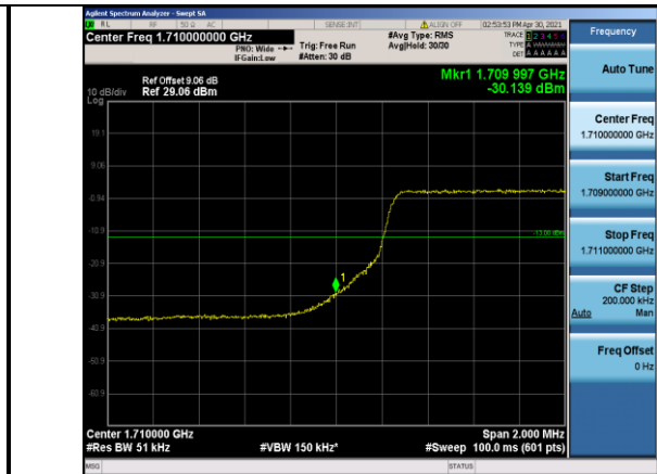
Band4-5MHz-16QAM-19975-25RB#0
