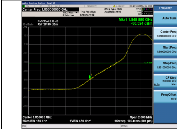
Band2-15MHz-QPSK-18675-1RB#0
