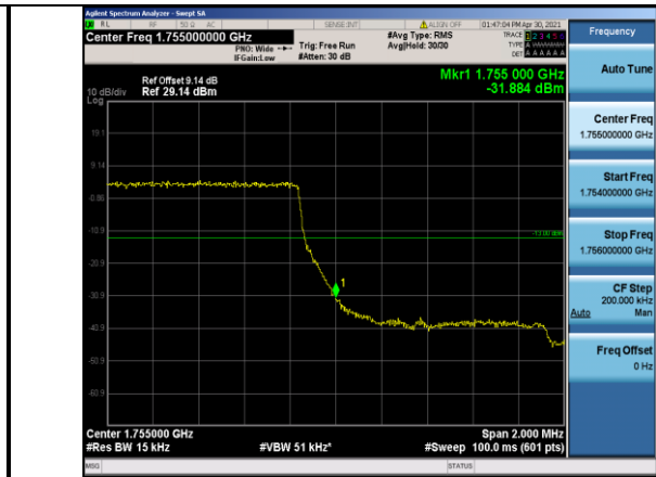
Band4-1.4MHz-QPSK-20393-6RB#0
