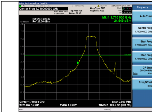
Band4-1.4MHz-QPSK-19957-1RB#0
