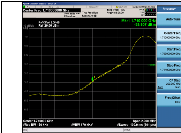
Band4-15MHz-16QAM-20025-1RB#0
