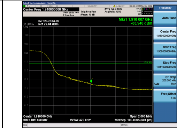
Band2-15MHz-QPSK-19125-75RB#0
