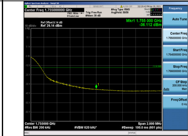
Band4-20MHz-16QAM-20300-100RB#0
