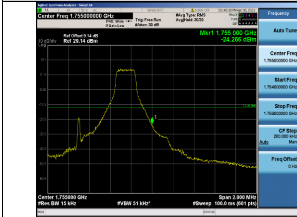
Band4-1.4MHz-QPSK-20393-1RB#5
