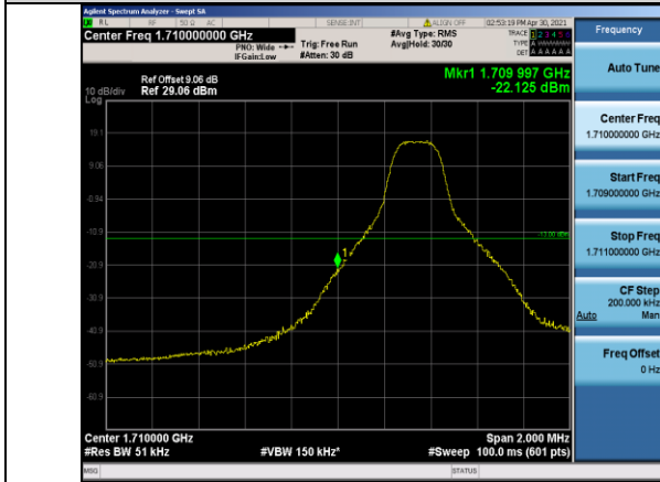
Band4-5MHz-16QAM-19975-1RB#0
