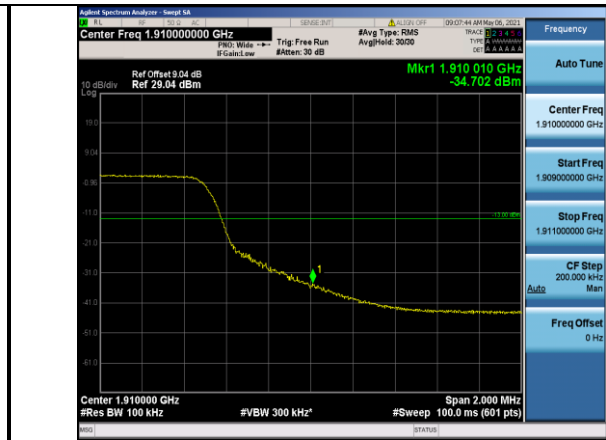
Band2-10MHz-QPSK-19150-50RB#0
