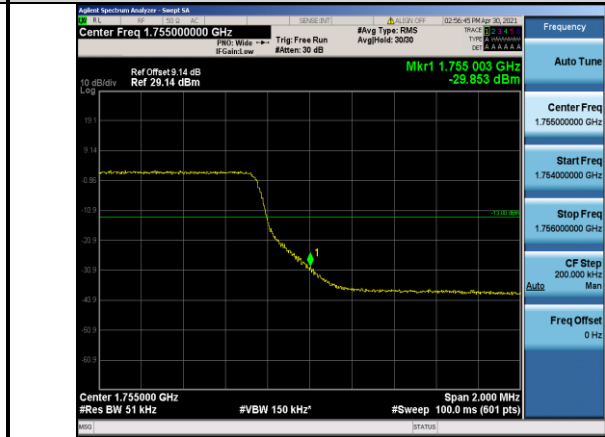
Band4-5MHz-16QAM-20375-25RB#0
