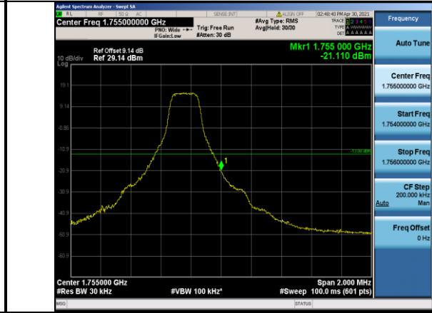
Band4-3MHz-QPSK-20385-1RB#14
