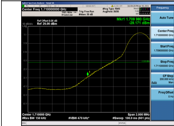
Band4-15MHz-QPSK-20025-1RB#0
