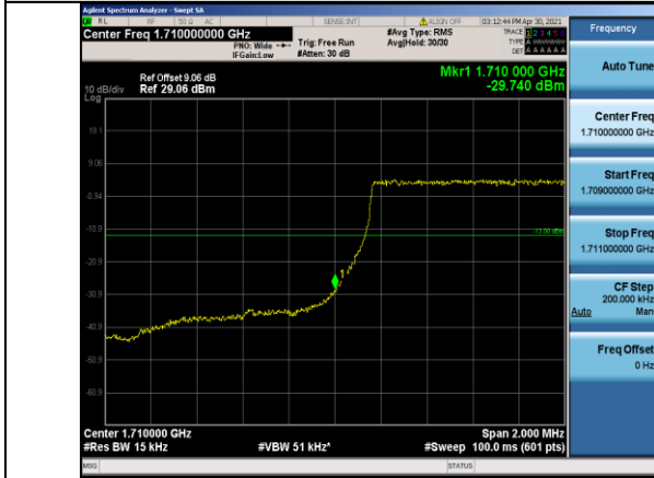
Band66-1.4MHz-QPSK-131979-6RB#0
