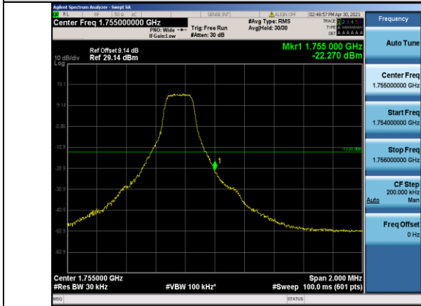
Band4-3MHz-16QAM-20385-1RB#14
