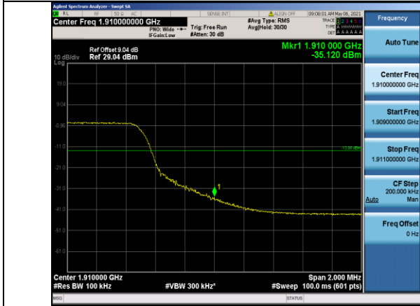
Band2-10MHz-16QAM-19150-50RB#0
