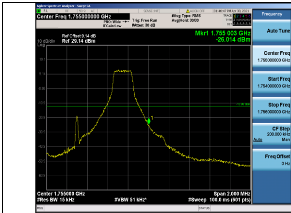
Band4-1.4MHz-16QAM-20393-1RB#5
