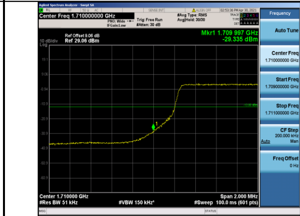
Band4-5MHz-QPSK-19975-25RB#0
