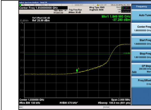
Band2-15MHz-16QAM-18675-75RB#0
