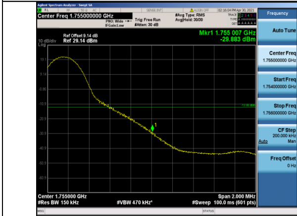
Band4-15MHz-16QAM-20325-1RB#74
