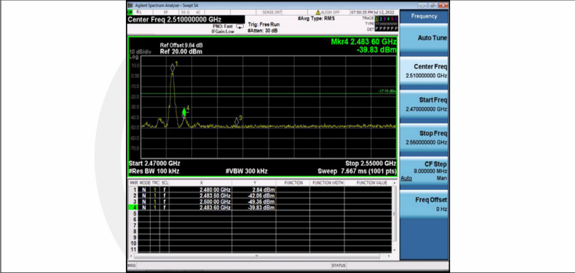
BLE_1M_Ant1_High_2480
