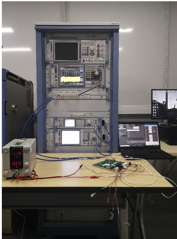
Photograph 3: Set-up photo for RF Conducted Singal test
