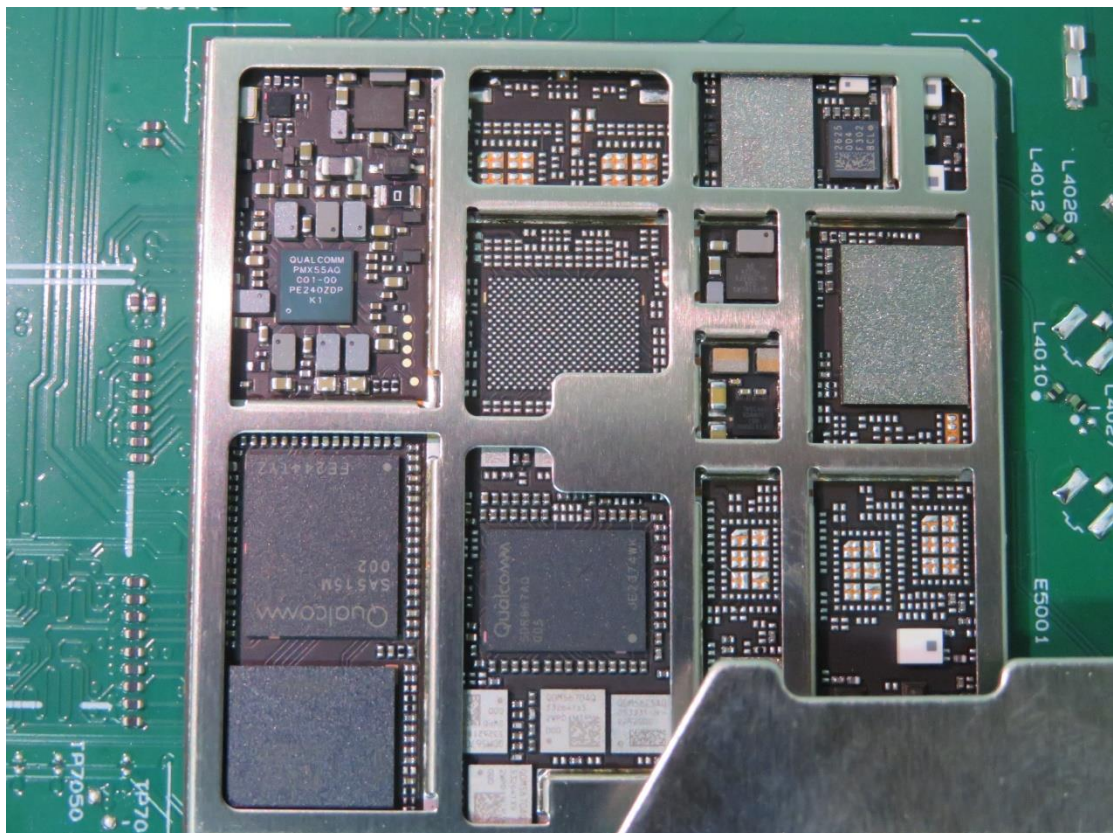
Internal View (The certificated module AN958-NA )
