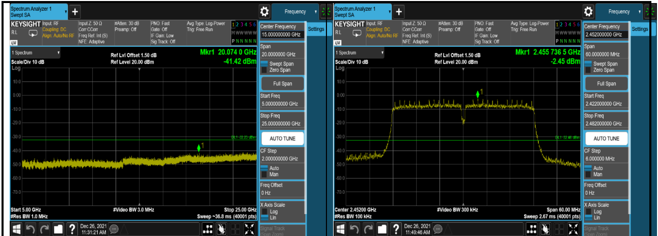
802.11n(HT40),2452MHz,Ant0,Plot 2,Band Edge
