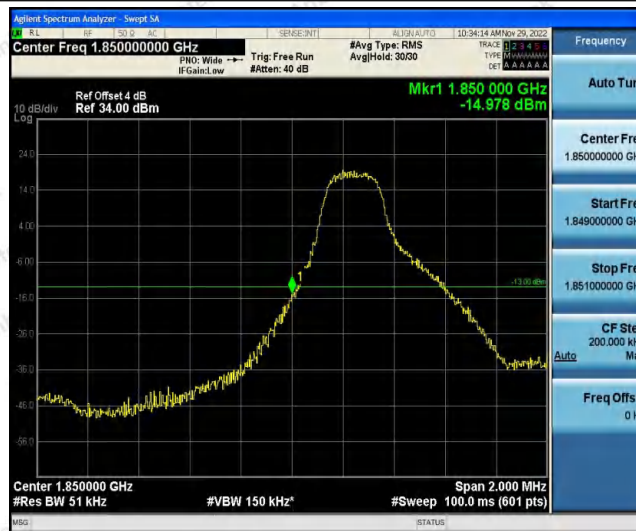
Band25-3MHz-16QAM-26055-1RB#14
