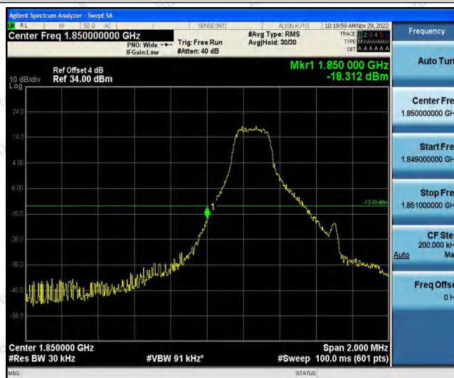
Band25-1.4MHz-QPSK-26047-1RB#5
