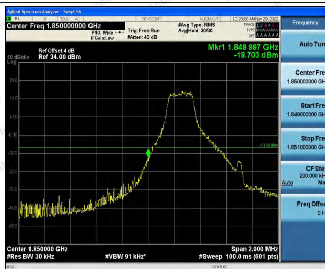
Band25-1.4MHz-16QAM-26047-1RB#5
