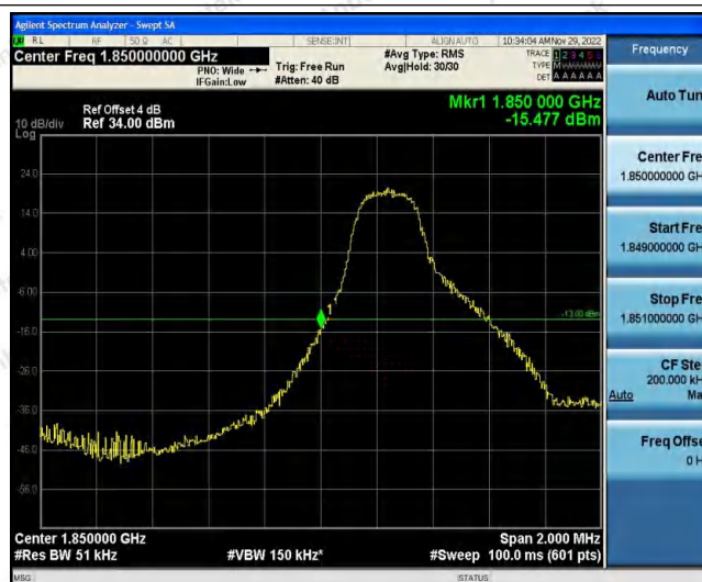
Band25-3MHz-QPSK-26055-1RB#14
