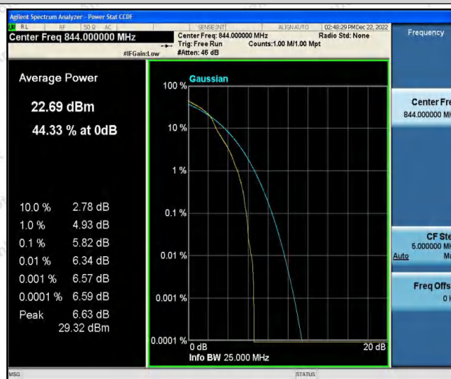
Band26-10MHz-16QAM-26990-50RB#0
