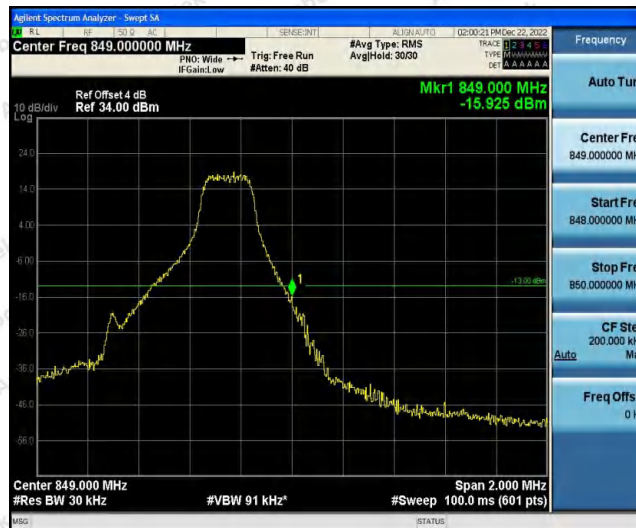
Band26-1.4MHz-16QAM-27033-6RB#0
