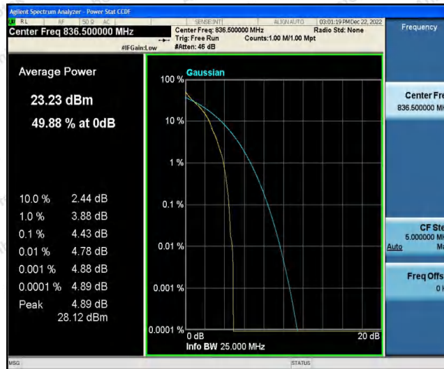
Band26-15MHz-QPSK-26915-75RB#0
