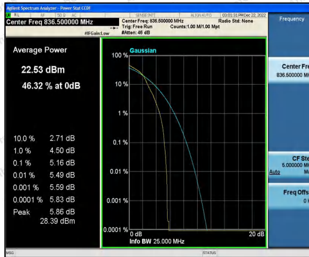
Band26-15MHz-16QAM-26915-75RB#0
