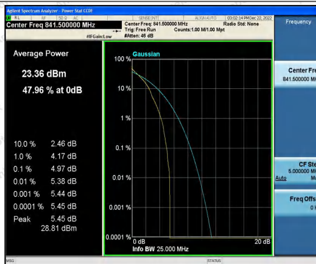
Band26-15MHz-QPSK-26965-75RB#0
