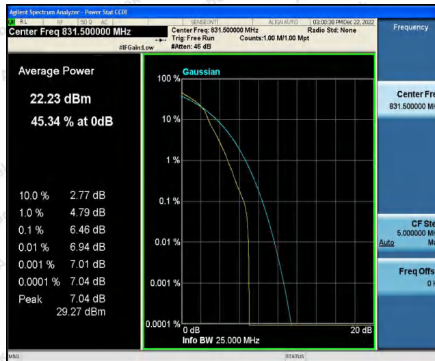
Band26-15MHz-16QAM-26865-75RB#0
