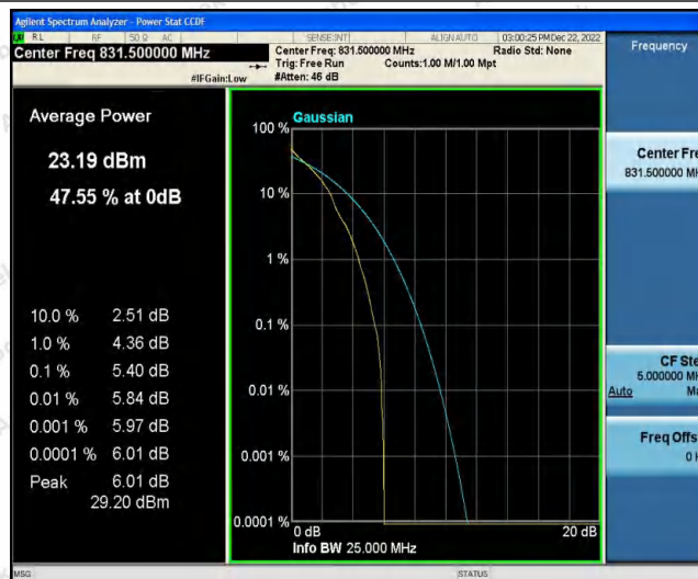
Band26-15MHz-QPSK-26865-75RB#0
