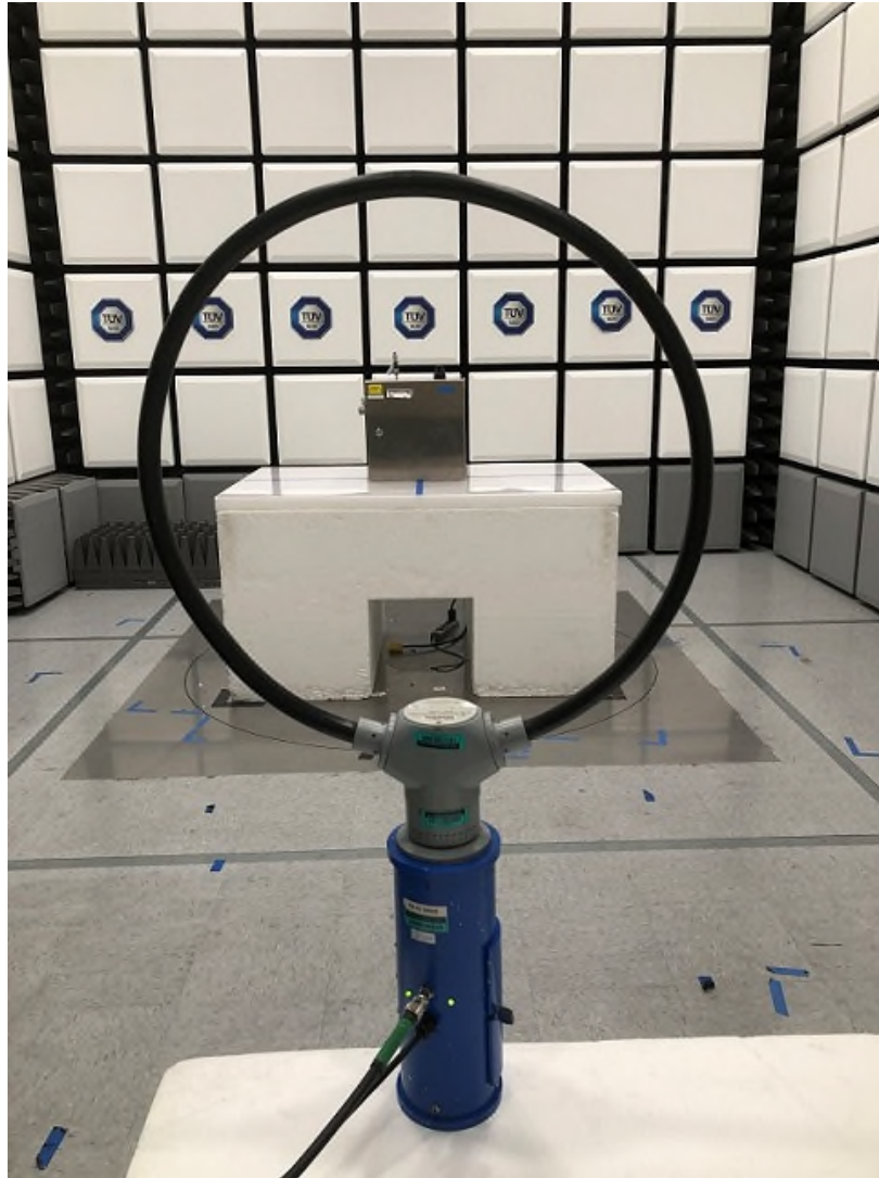
Radiated Emissions Below 30 MHz
