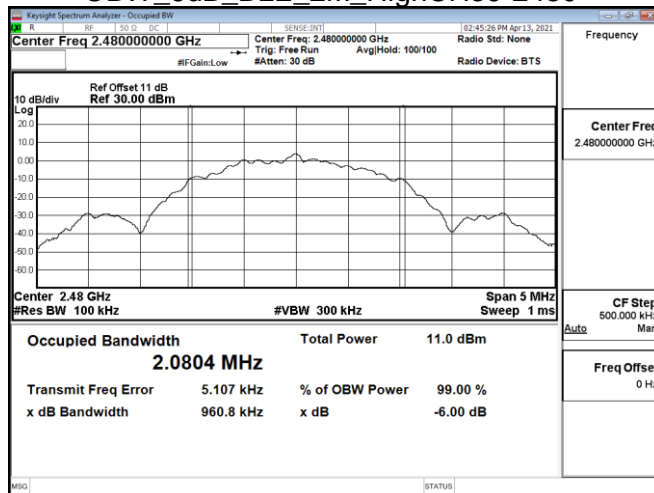
OBW_6dB_BLE_2M_HighCH39-2480
