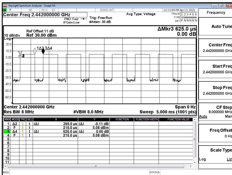
Duty Cycle_BLE_1M_MidCH20-2442
