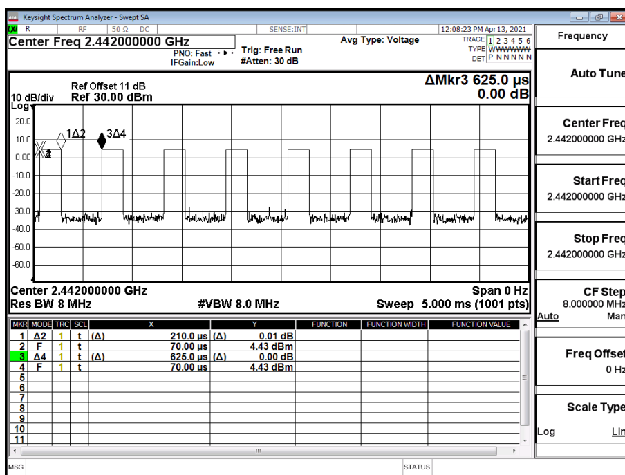
Duty Cycle_BLE_2M_MidCH20_2442
