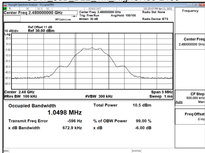
OBW_6dB_BLE_1M_HighCH39-2480
