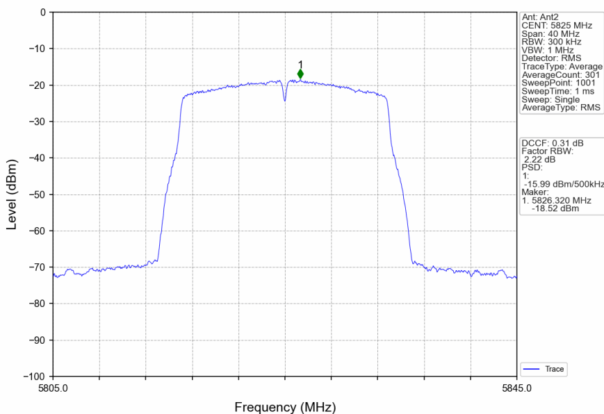
802.11ac(VHT20)_HCH_5825MHz_MIMO_NTNV
