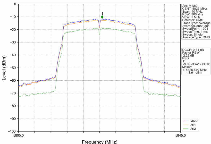
802.11ac(VHT20)_HCH_5825MHz_MIMO_NTNV
