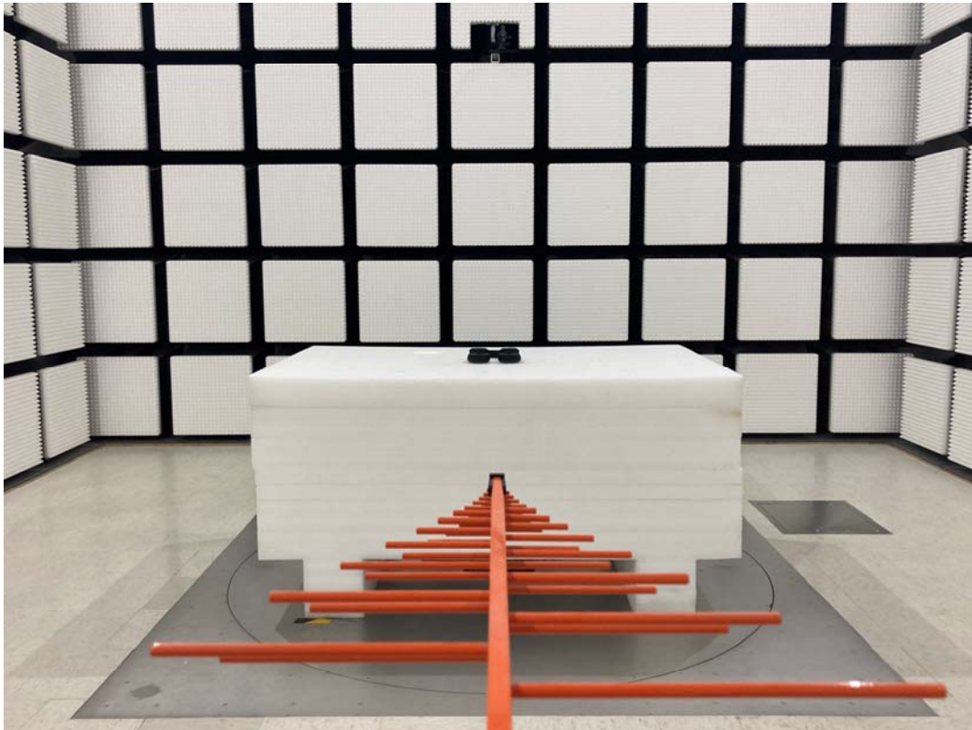
Radiated Emission Below 1GHz View - WH304A
