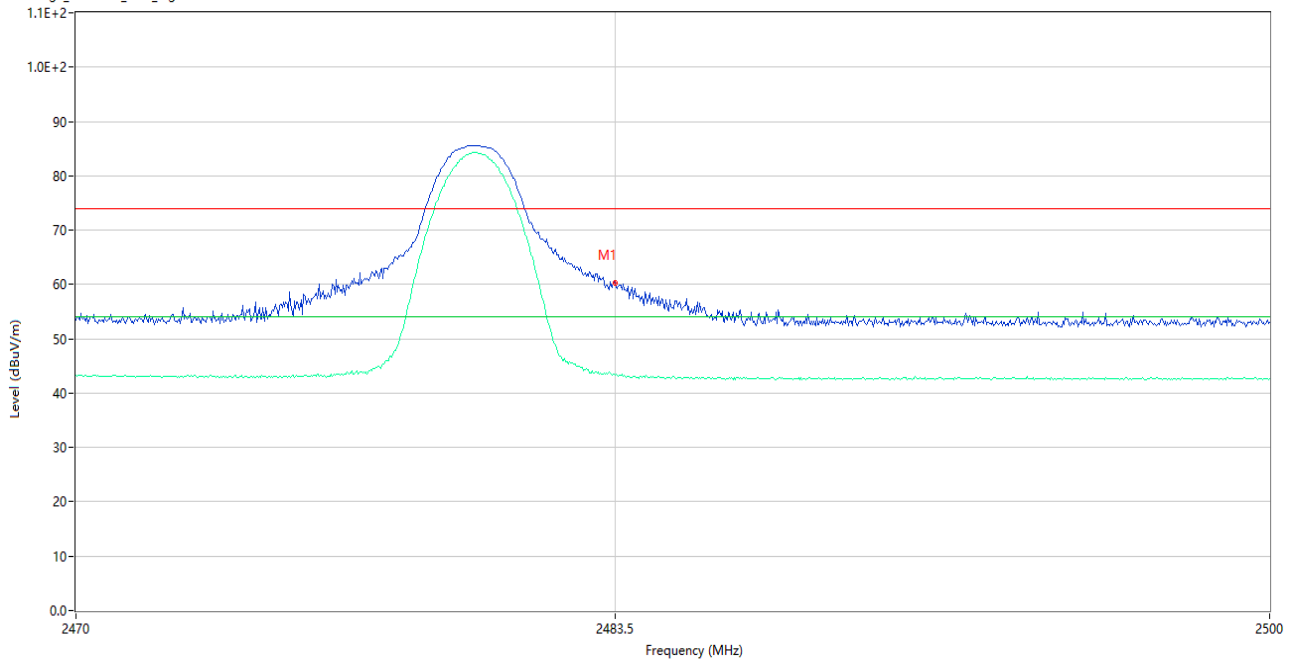
Bandedge_FCC-WIFI_2.4G_Right
