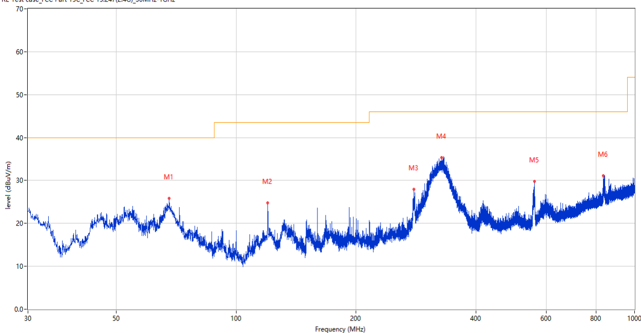
RE Test case_FCC Part 15C_FCC 15.247(2.4G)_30MHz-1GHz
