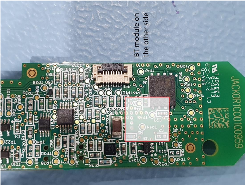
BT module back view
