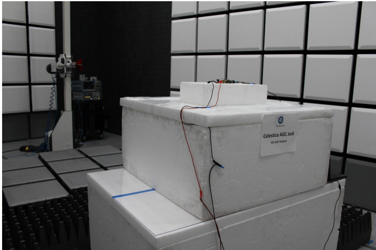
Radiated Emissions Test Setup (1GHz to 18GHz)
