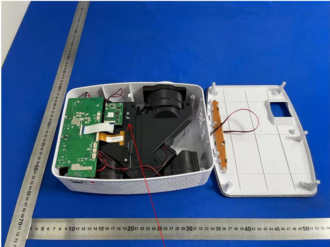
WiFi Antenna
