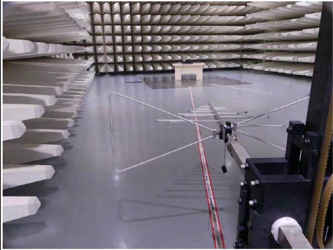
Test setup up to 1 GHz horizontal polarization
