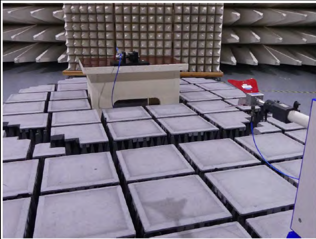
Test setup above 1 GHz vertical polarization
