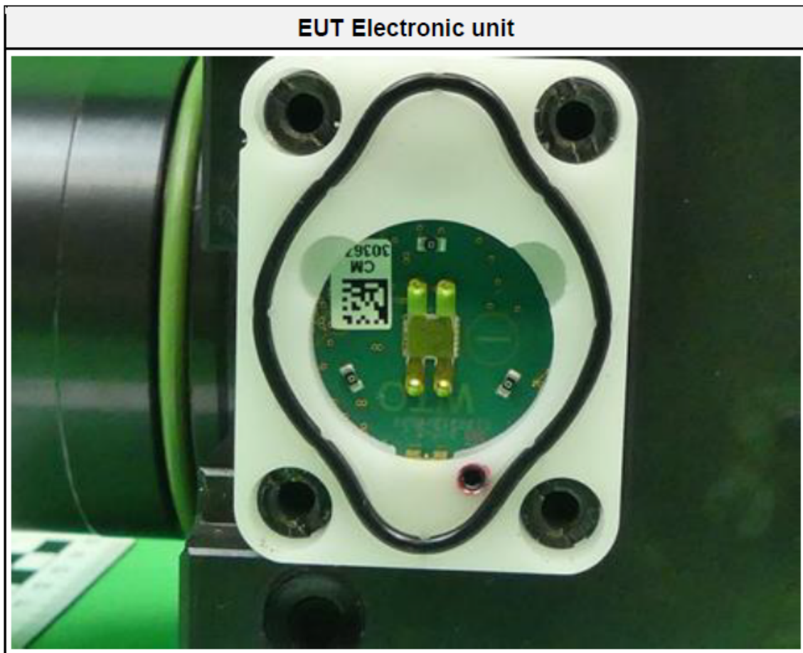
Bluetooth module top view
