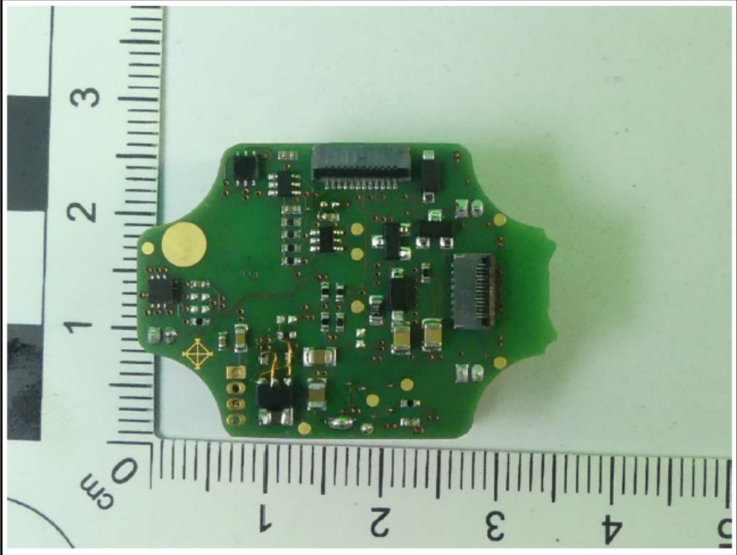
EUT PCB Bluetooth top view
