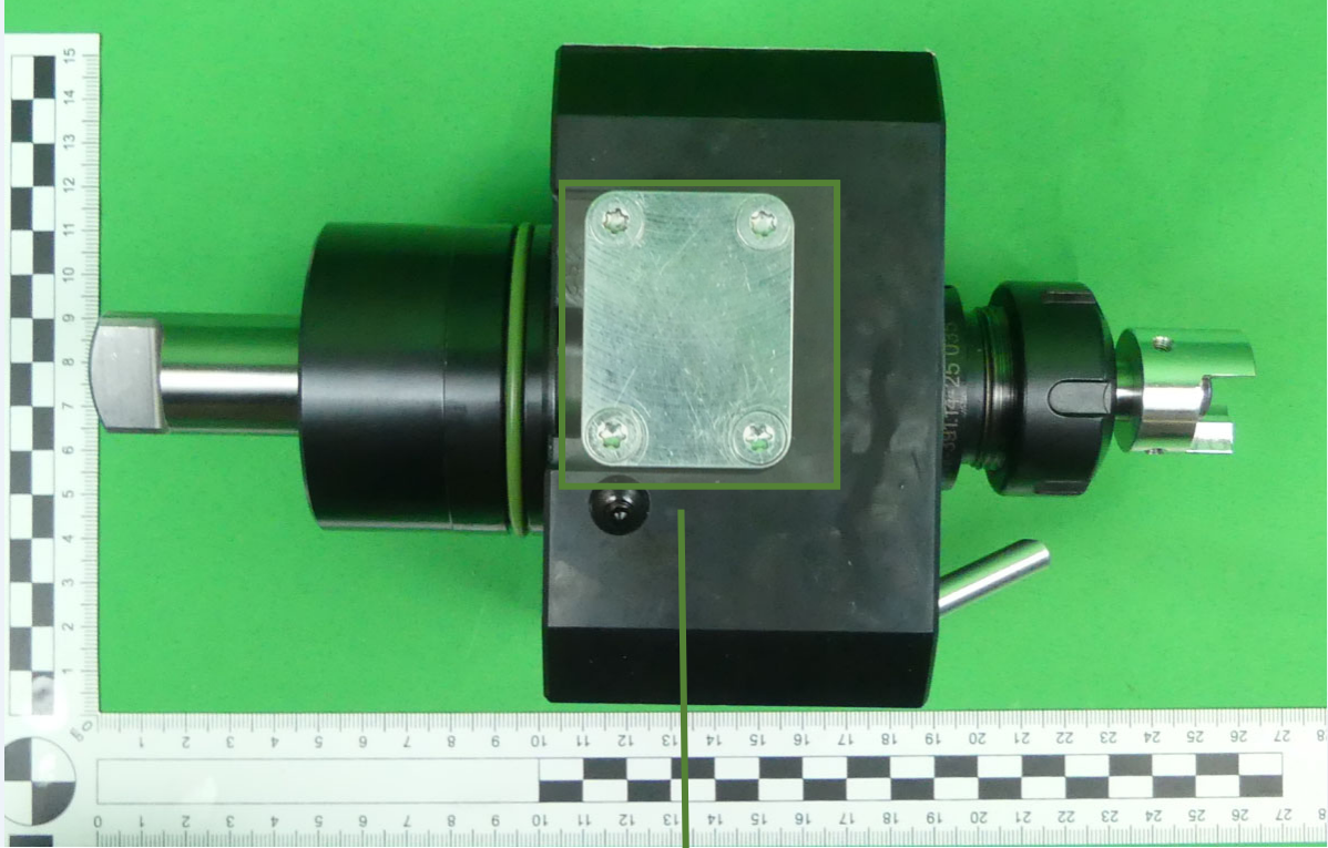
EUT: WTO SC 002 (mounted on tool holder)
