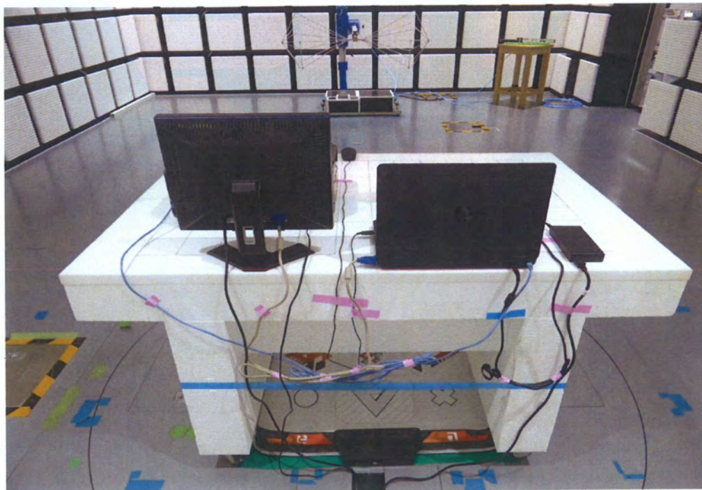
Bluetooth Mode
