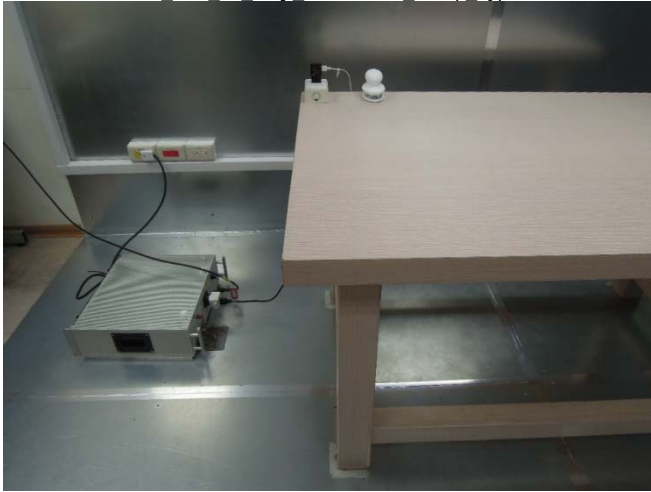
FCC Part 15 C QI Conduction Setup Type A
