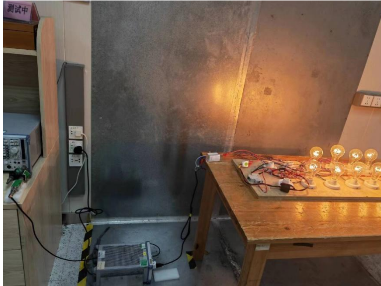
CONDUCTED EMISSION TEST
