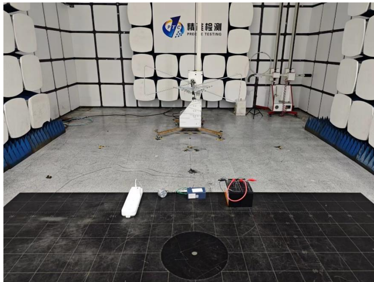
Test Frequency From Below 30MHz
