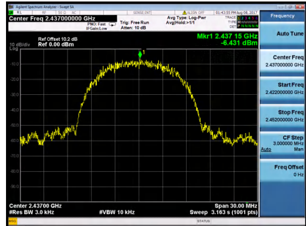
Channel 6 (2437MHz)
