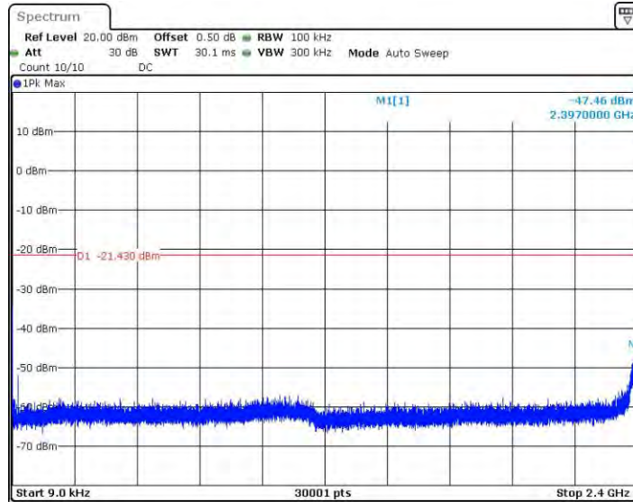
11AX40SISO_Ant1_2422_0.009~2400
