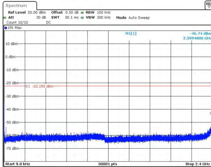
11AX40SISO_Ant0_2422_0.009~2400
