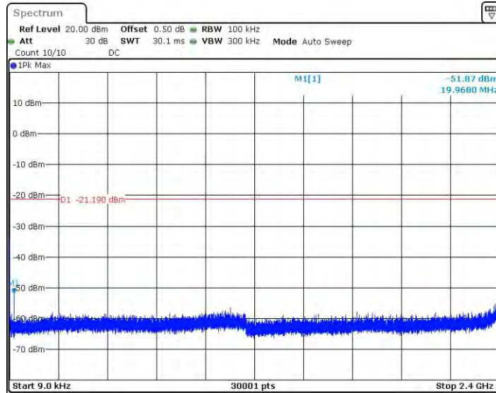
11AX40SISO_Ant1_2452_0.009~2400
