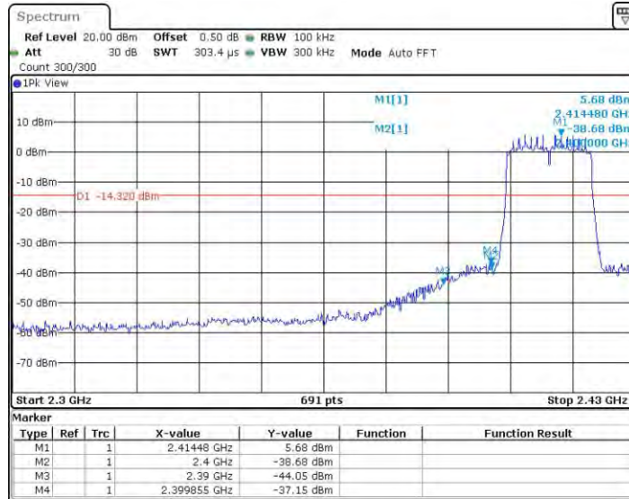
11N20SISO_Ant0_Low_2412
