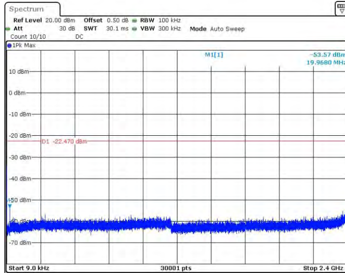
11AX40SISO_Ant0_2452_0.009~2400
