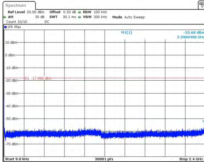
11AX20SISO_Ant1_2437_0.009~2400
