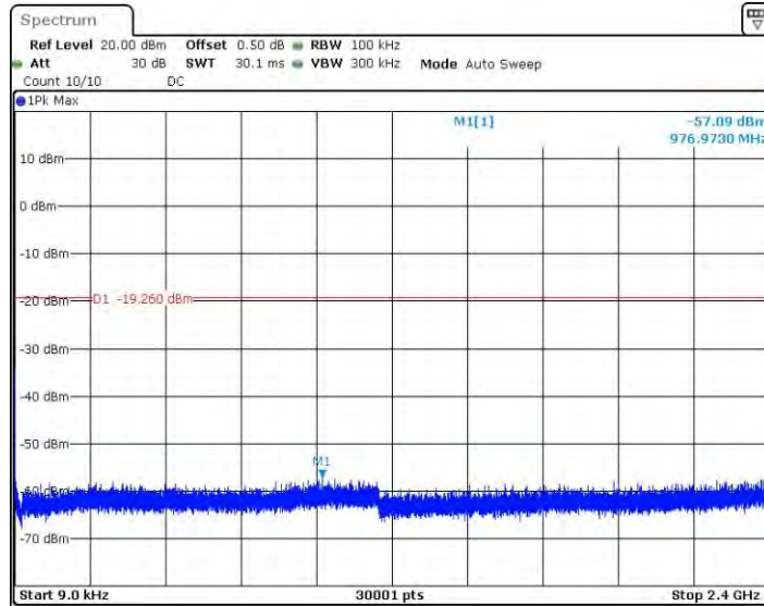
11AX20SISO_Ant0_2462_0.009~2400
