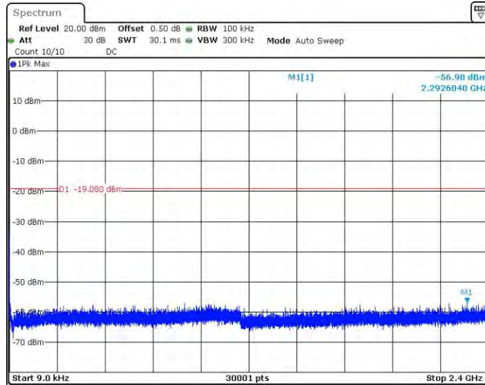
11AX20SISO_Ant0_2437_0.009~2400
