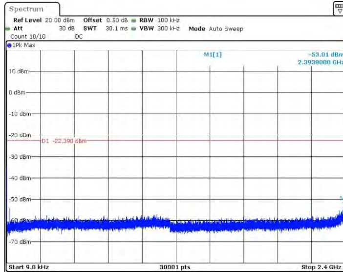
11AX40SISO_Ant0_2437_0.009~2400
