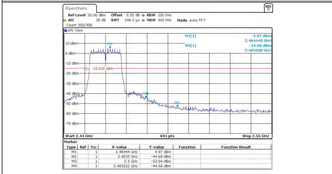
11G_Ant0_High_2462
