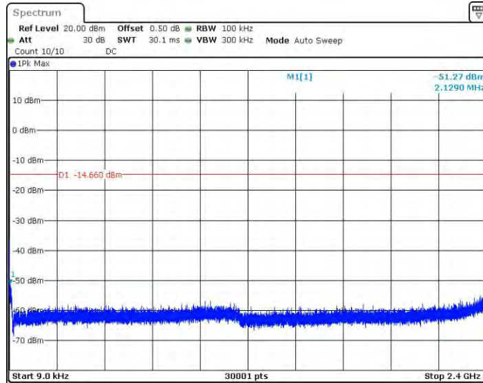
11G_Ant0_2437_0.009~2400
