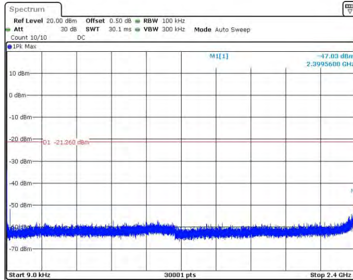
11AX40SISO_Ant1_2437_0.009~2400
