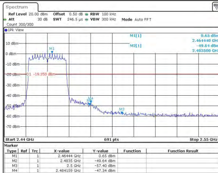
11AX20SISO_Ant0_High_2462
