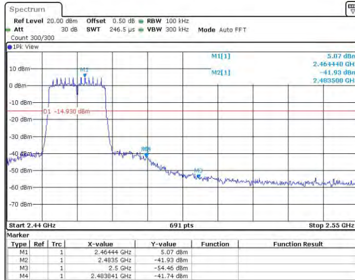
11N20SISO_Ant0_High_2462
