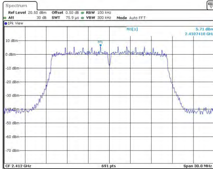
11G_Ant0_2412_0~Reference
