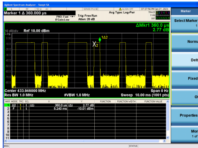
(Time per burst: 0.360ms*18pcs)
