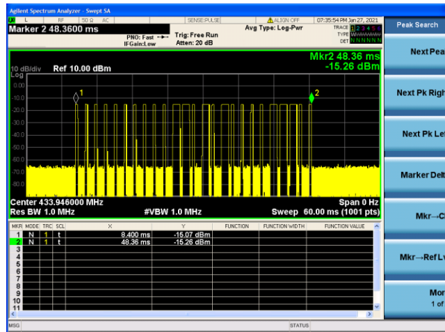
(Total Bursts in a transmit cycle 25pcs)
