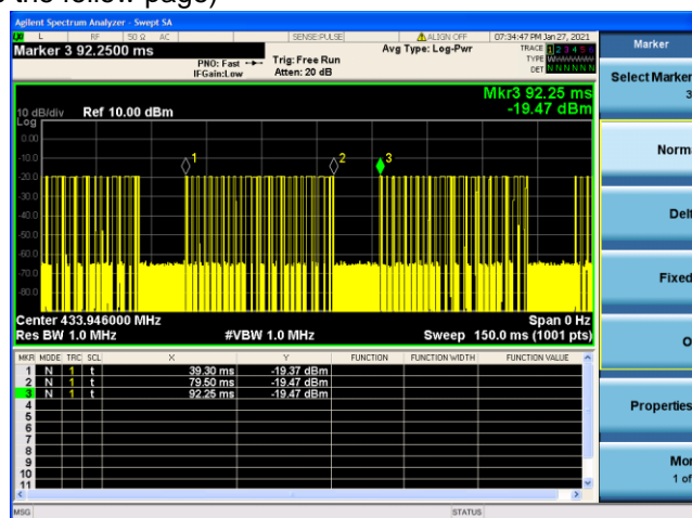
(Transmit cycle 52.95ms)
