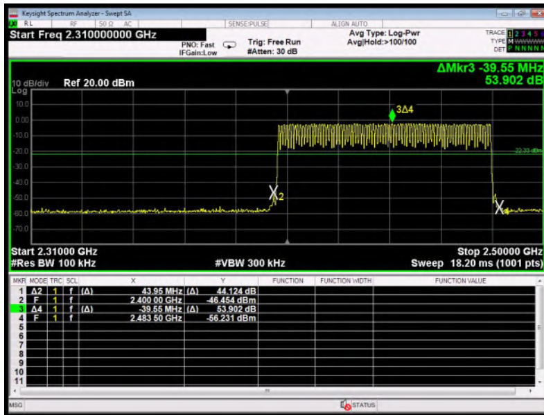
BDR mode
