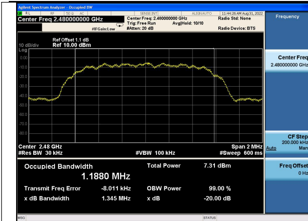
Test Mode:π/4QPSK(2DH5) 2480MHz
