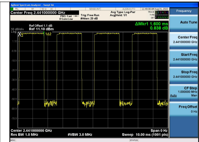
Test Mode:π/4DQPSK(2DH3) 2441MHz
