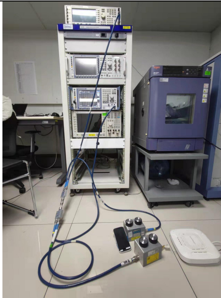
Dynamic Frequency Selection Test setup
