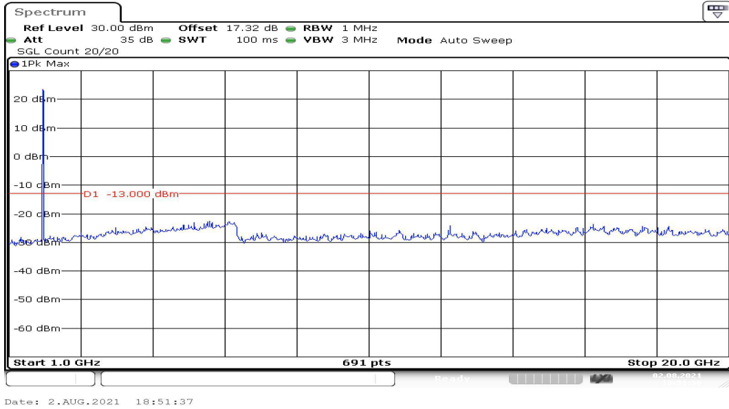
Channel 9400 1GHz~20GHz(dBm) Note: The signal beyond the limit is the signal transmitted by EUT.
