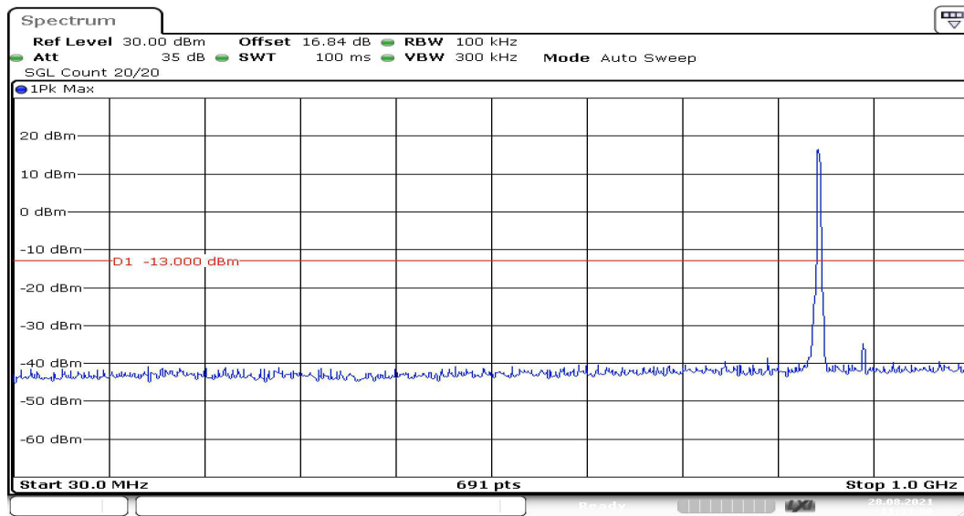
Channel 4183 30MHz~1GHz(dBm)
