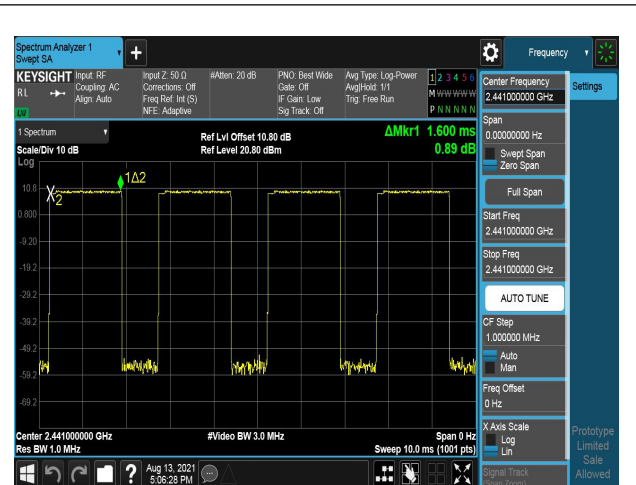
Modulation: \pi/4 DQPSK 2DH3 2441MHz
