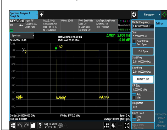
Modulation: GFSK DH5 2441MHz
