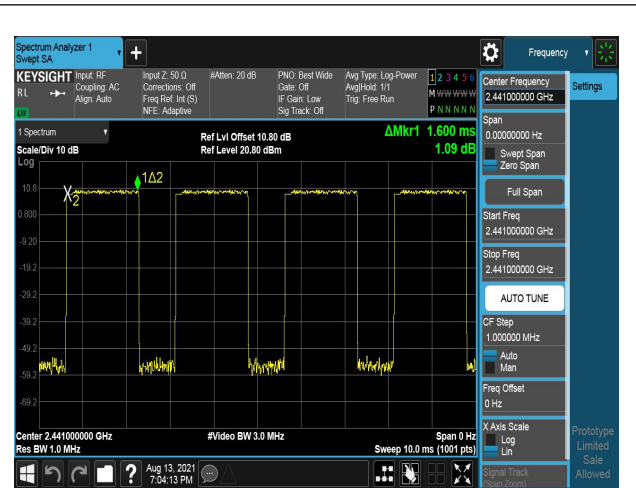
Modulation: 8DPSK 3DH3 2441MHz
