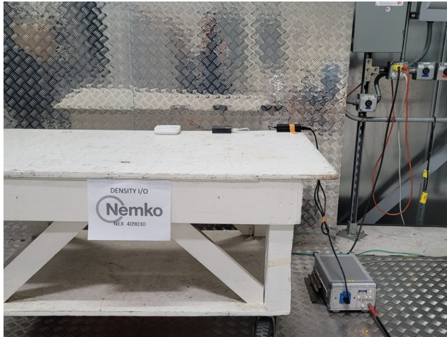
Figure 4 – AC conducted emissions test setup, front view
