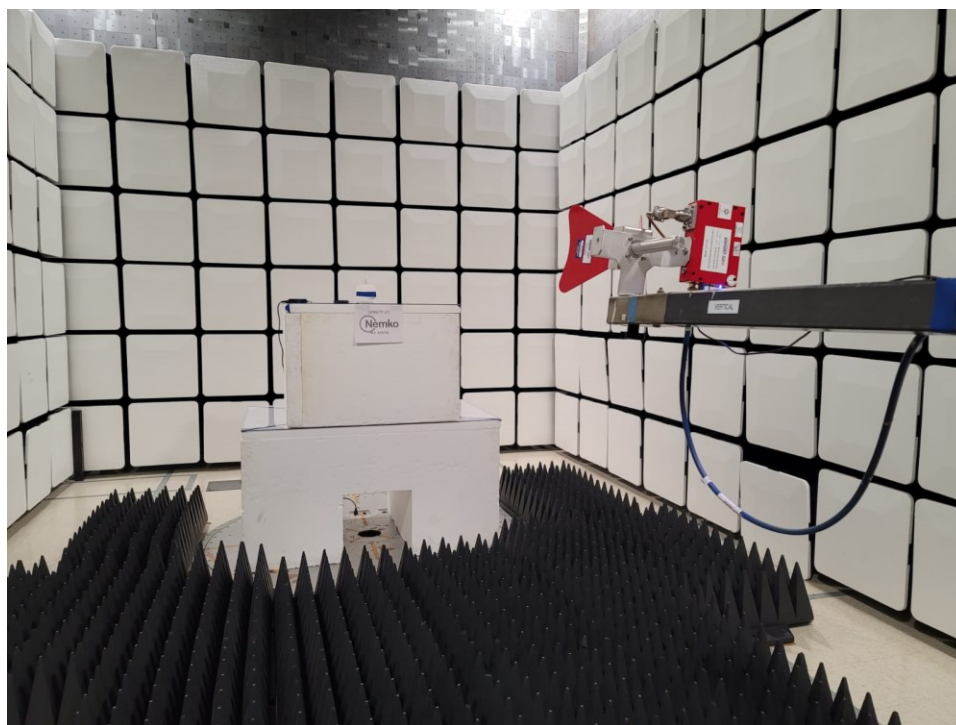
Figure 2 - Radiated emissions 1 – 40 GHz, front view
