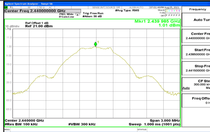
BLE_1M_Ant1_2440_0~Reference
