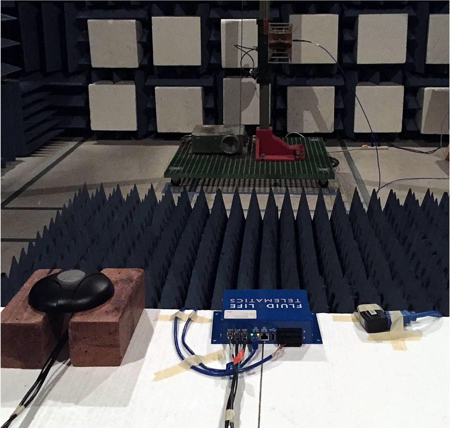
Figure 3: Unwanted Radiated Emissions (over 1GHz) Test Setup
