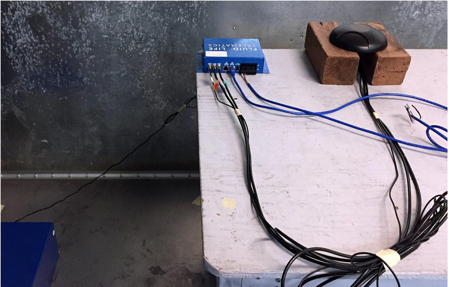
Figure 1: Conducted emissions
