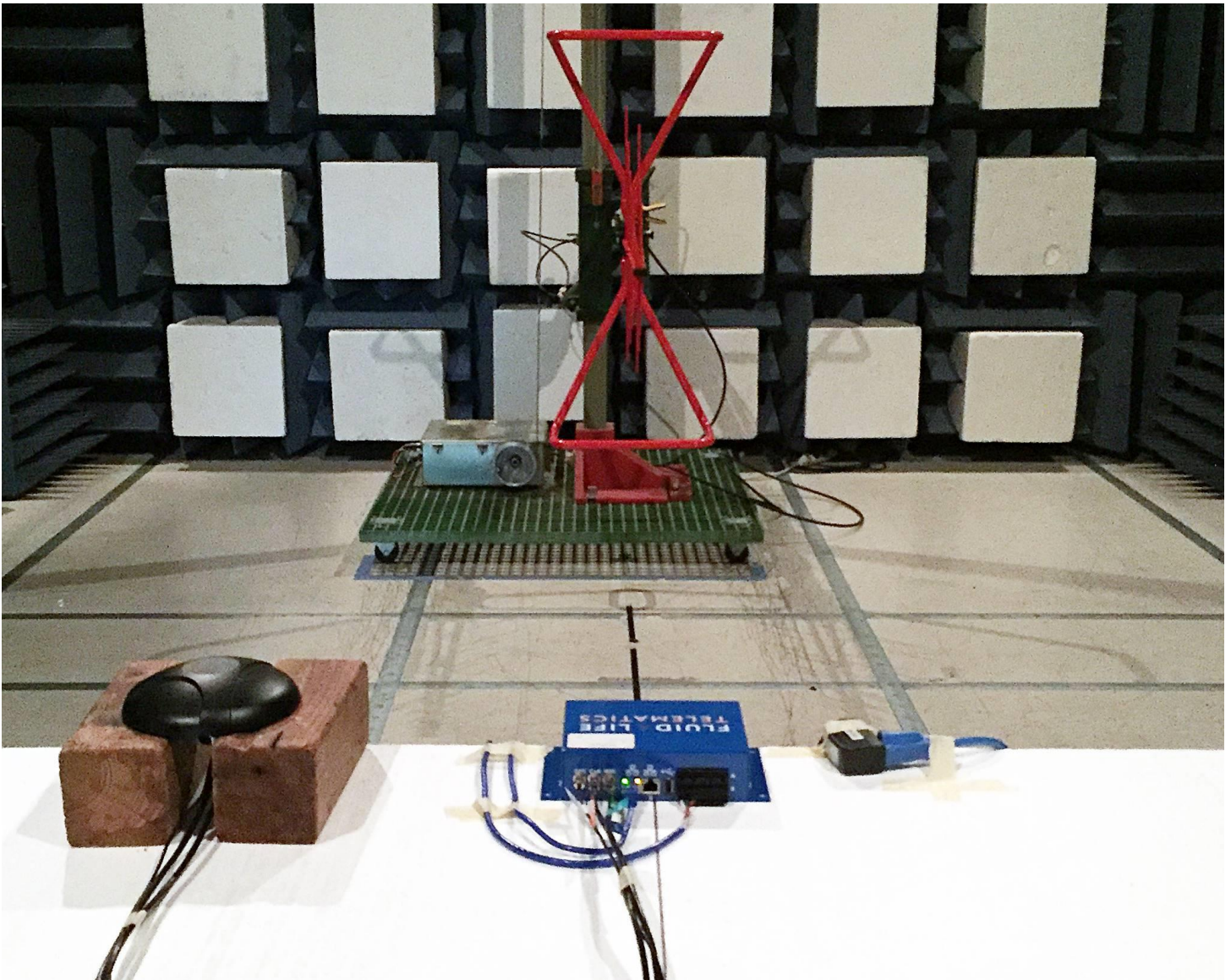
Figure 2: Unwanted Radiated Emissions (30 to 1000MHz) Test Setup
