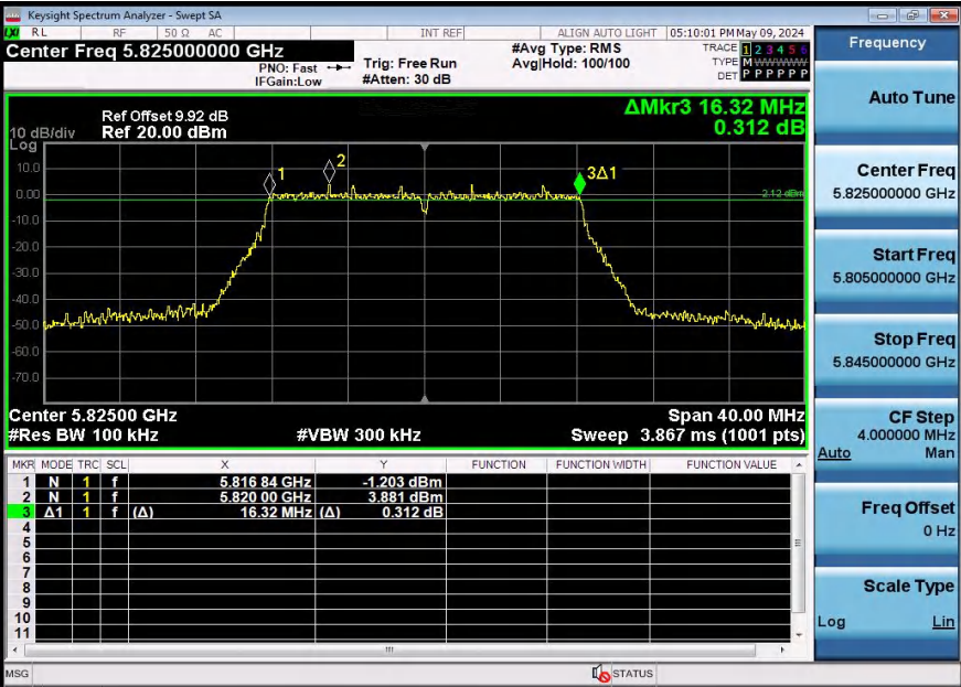
11A-5825-PASS
