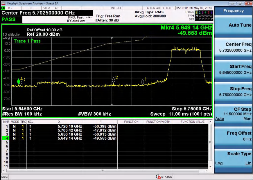
11AC20SISO-5745-PASS
