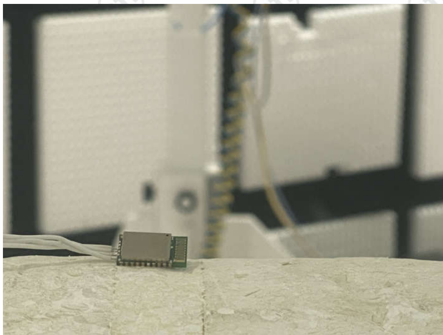
Radiated spurious emission Test Setup-4(Above 1GHz)close up photo
