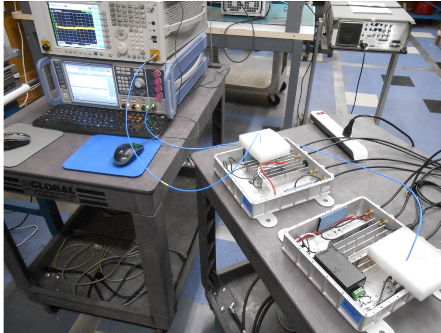
Conducted RF (1)
