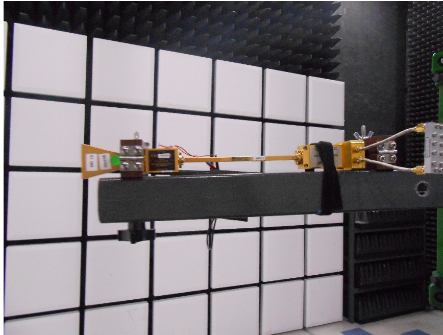
Radiated Emission_50 - 75 GHz (5)
