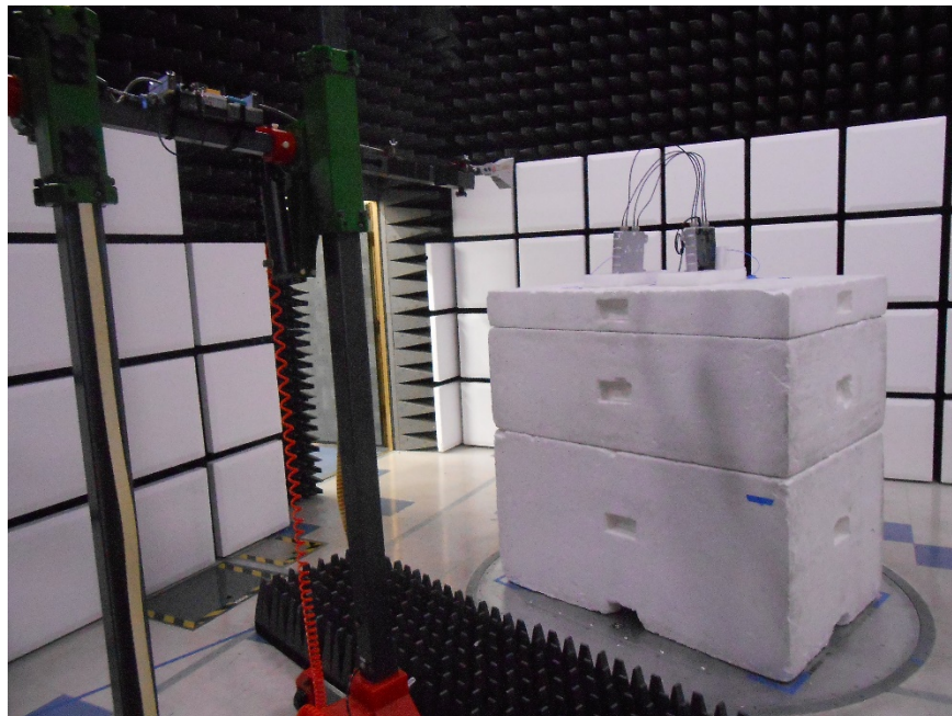
Radiated Emission_18 - 40 GHz (2)
