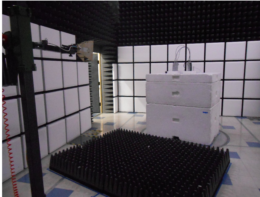
Radiated Emission_1 - 18 GHz (1)
