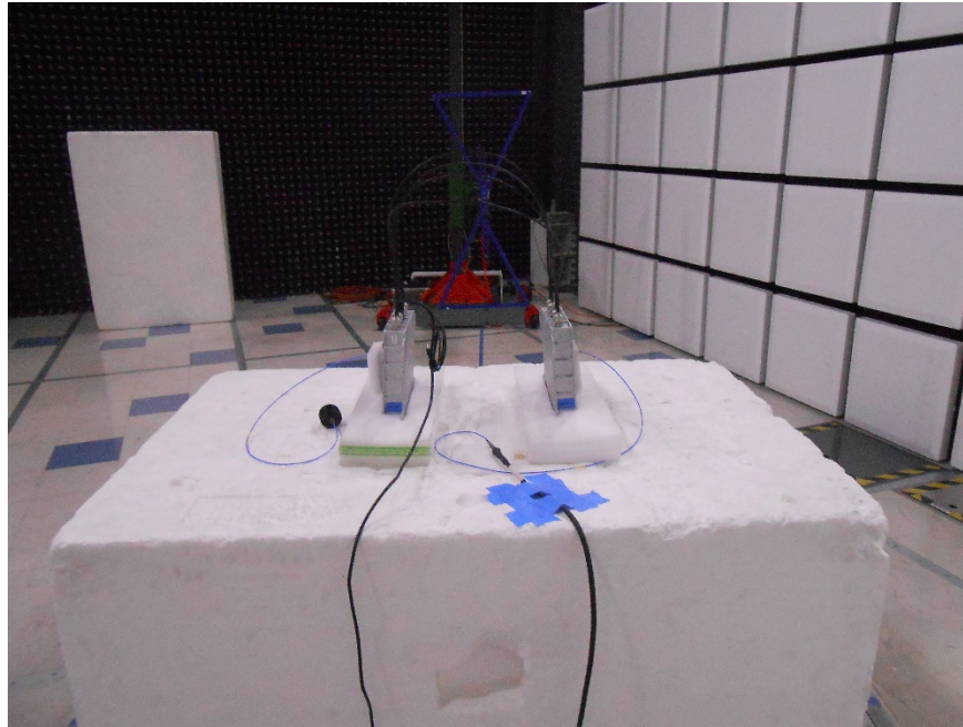
Radiated Emission_30 - 1000 MHz (3)
