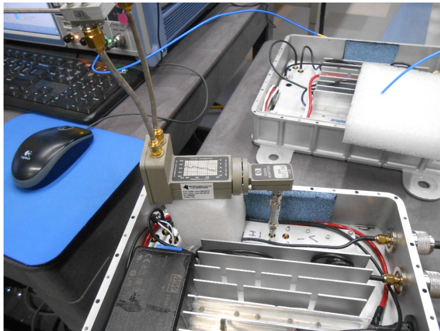
Conducted RF_40 - 50 GHz (4)
