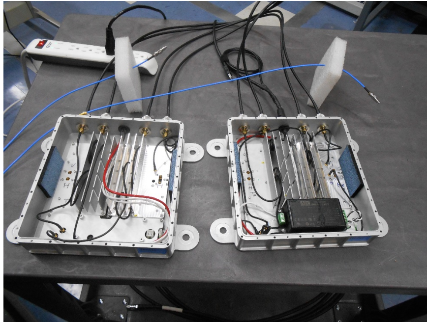
Conducted RF (3)
