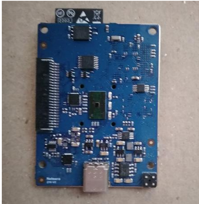
Photograph No.1 130H-Plus / 131H-Plus PCB Component side
