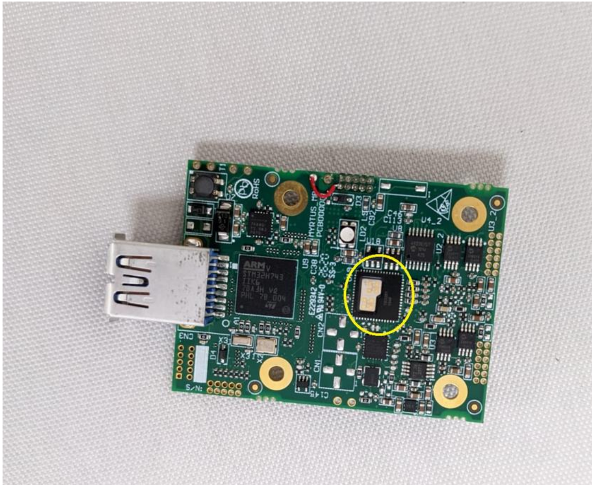
Photograph No.1 130H / 131H / 130W / 131W PCB front view
