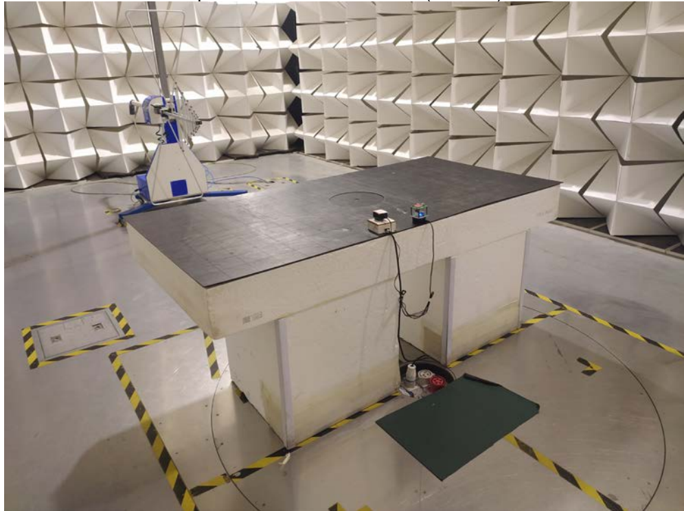
Spurious Emissions Radiated(30M-1G)
