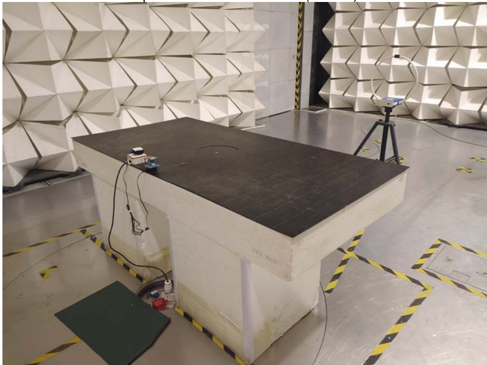
Spurious Emissions Radiated(9k-30M)
