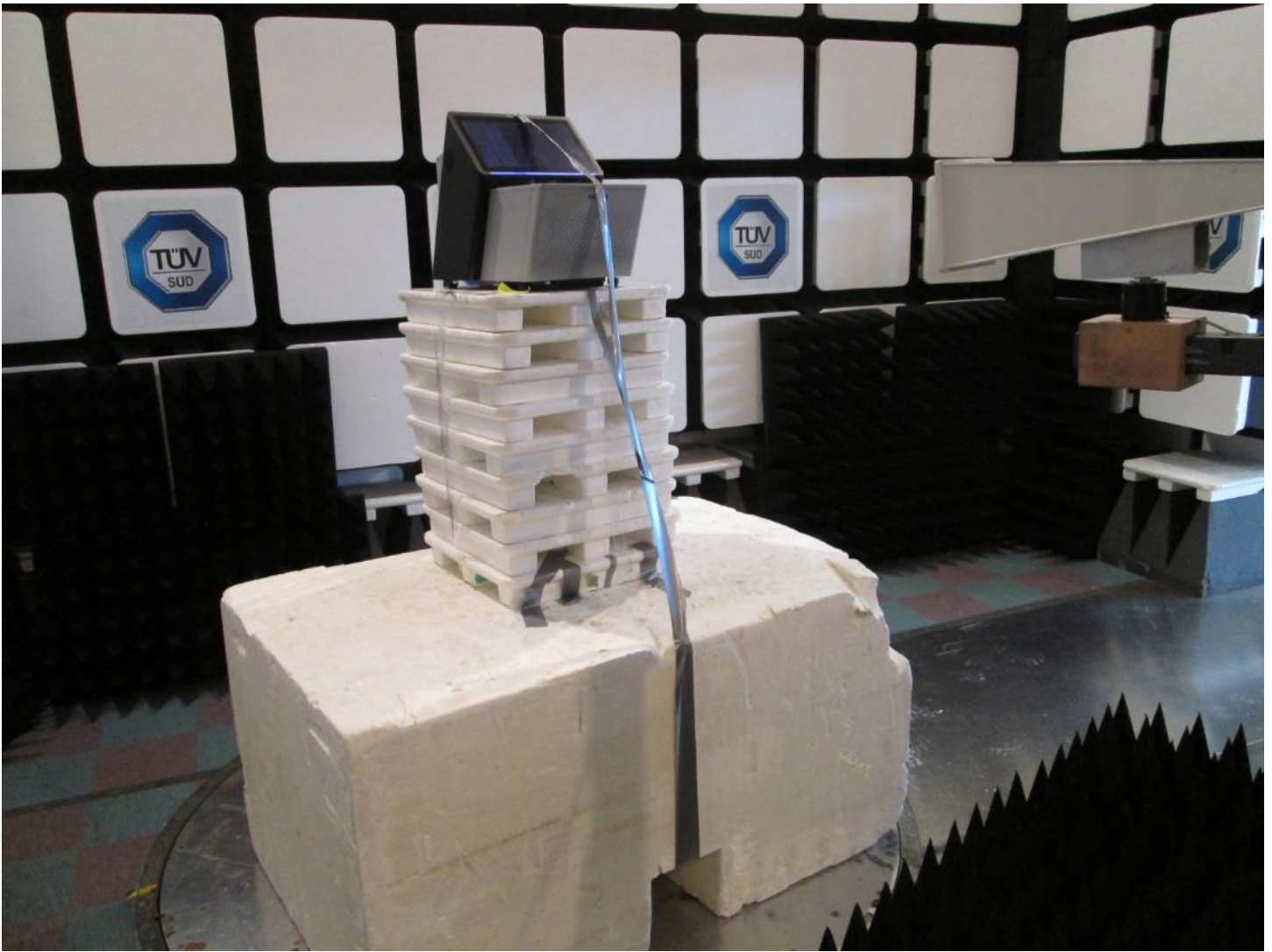
Test setup photo 5 Radiated measurements, 10 GHz – 18 GHz
