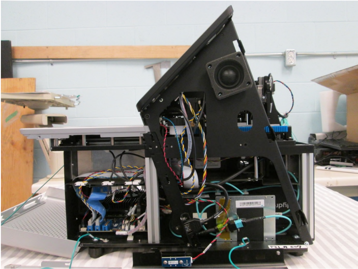
EUT – Internal view 2 Panels opened, left side
