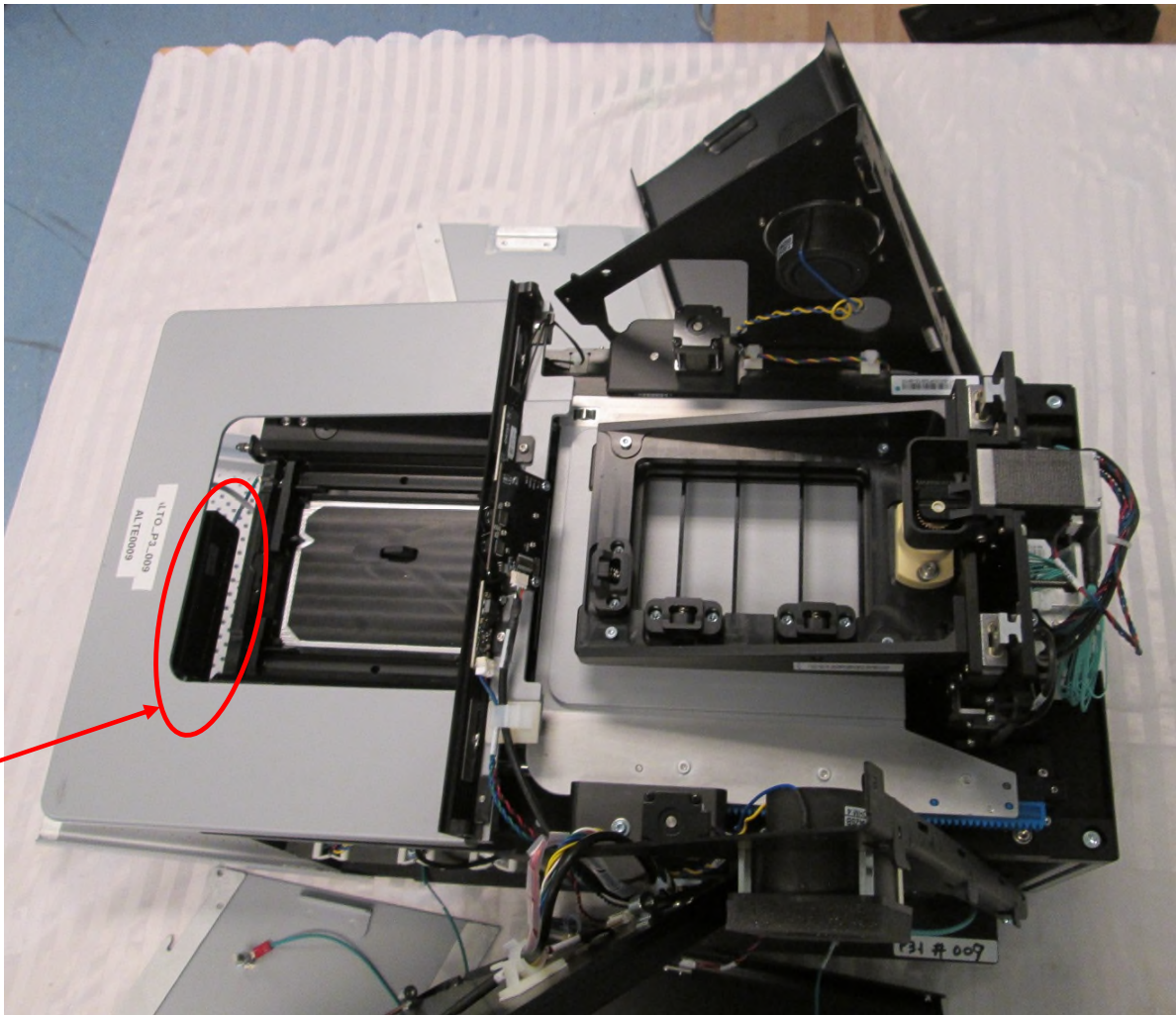
EUT – Internal view 7 Panels opened, left side, monitor detached
