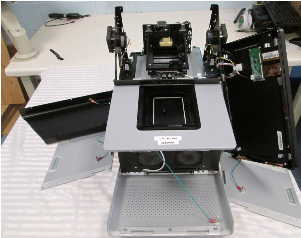
EUT – Internal view 6 Panels opened, front, monitor detached
