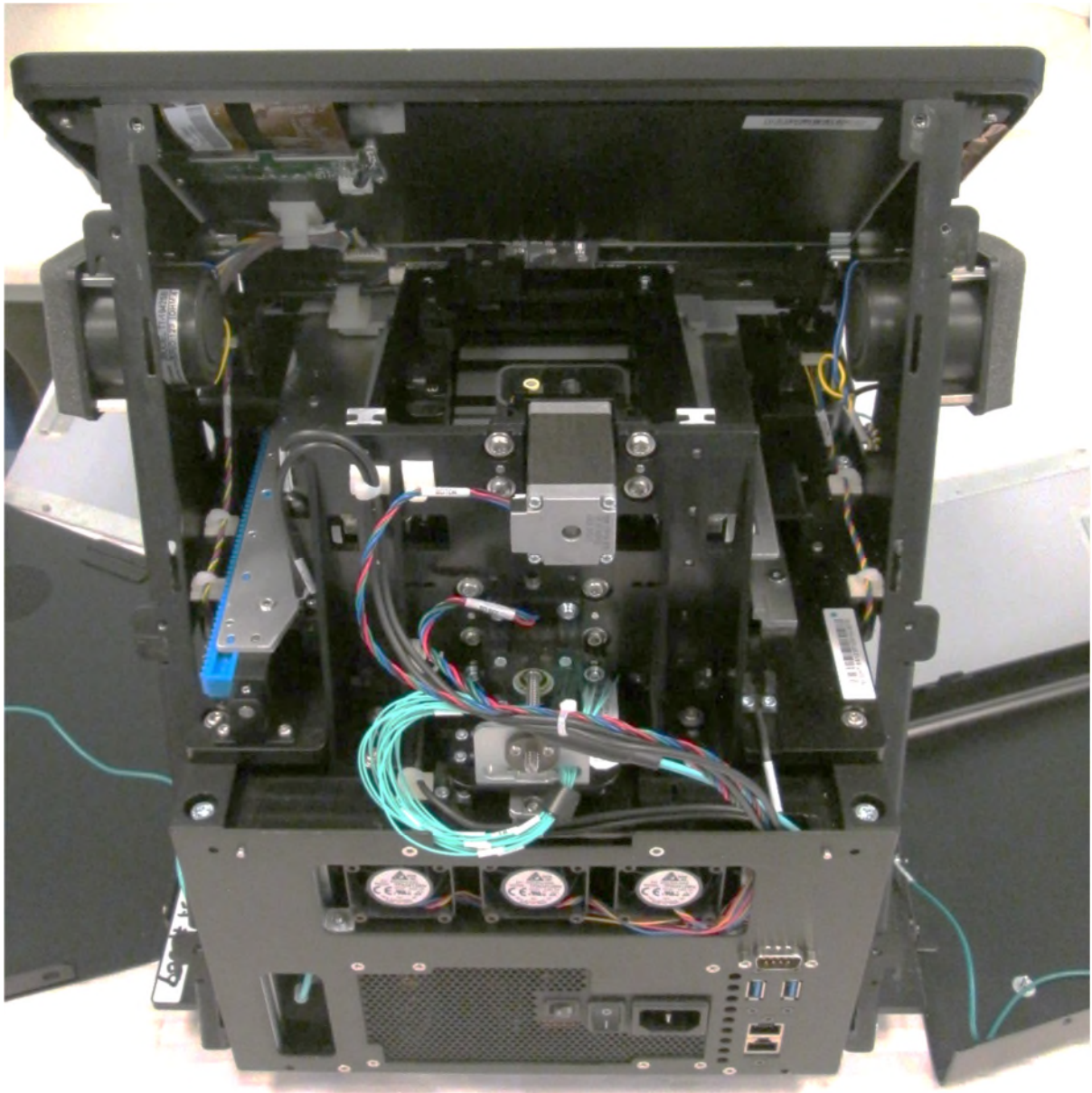
EUT – Internal view 4 Panels opened, back
