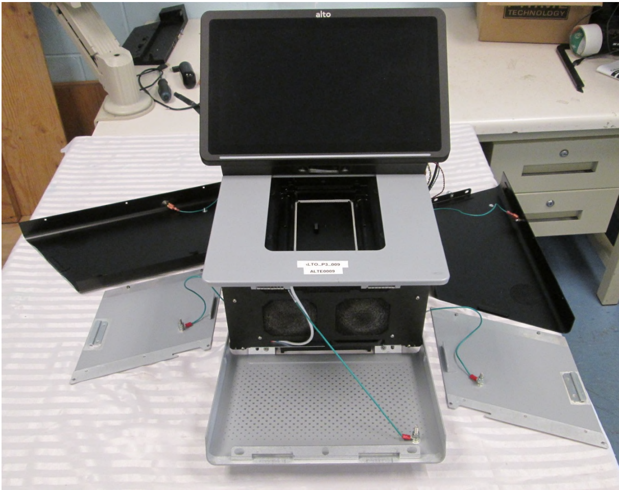
EUT – Internal view 1 Panels opened, front
