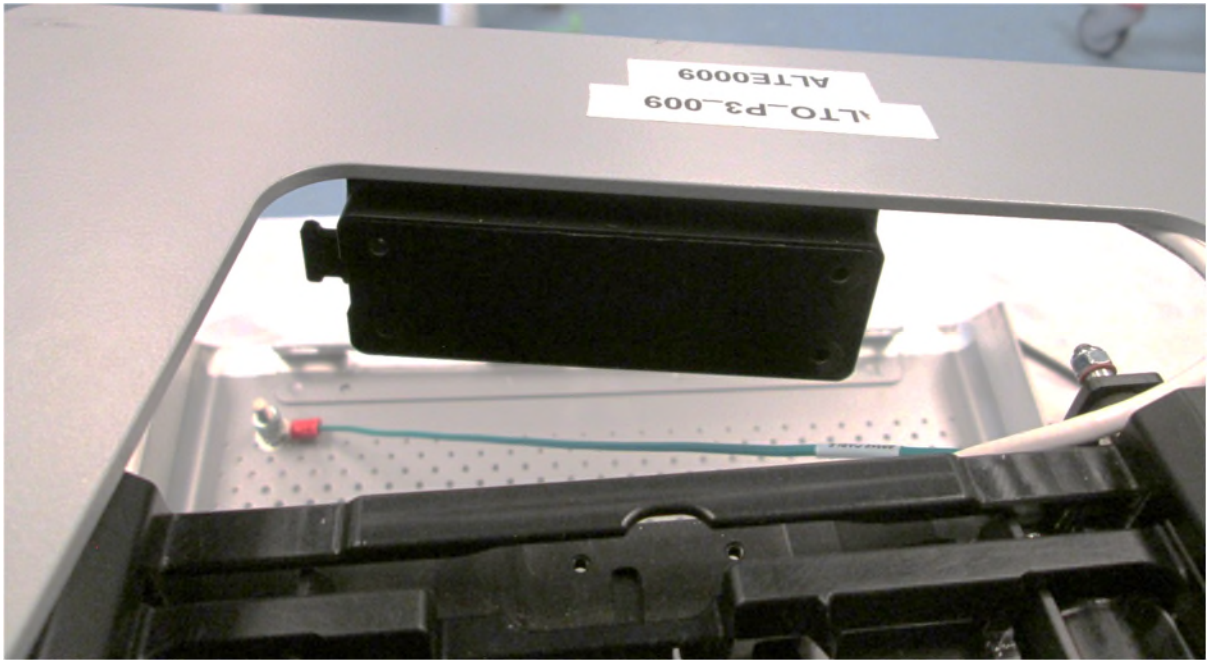
EUT – Internal view 8 NFC board compartment close-up
