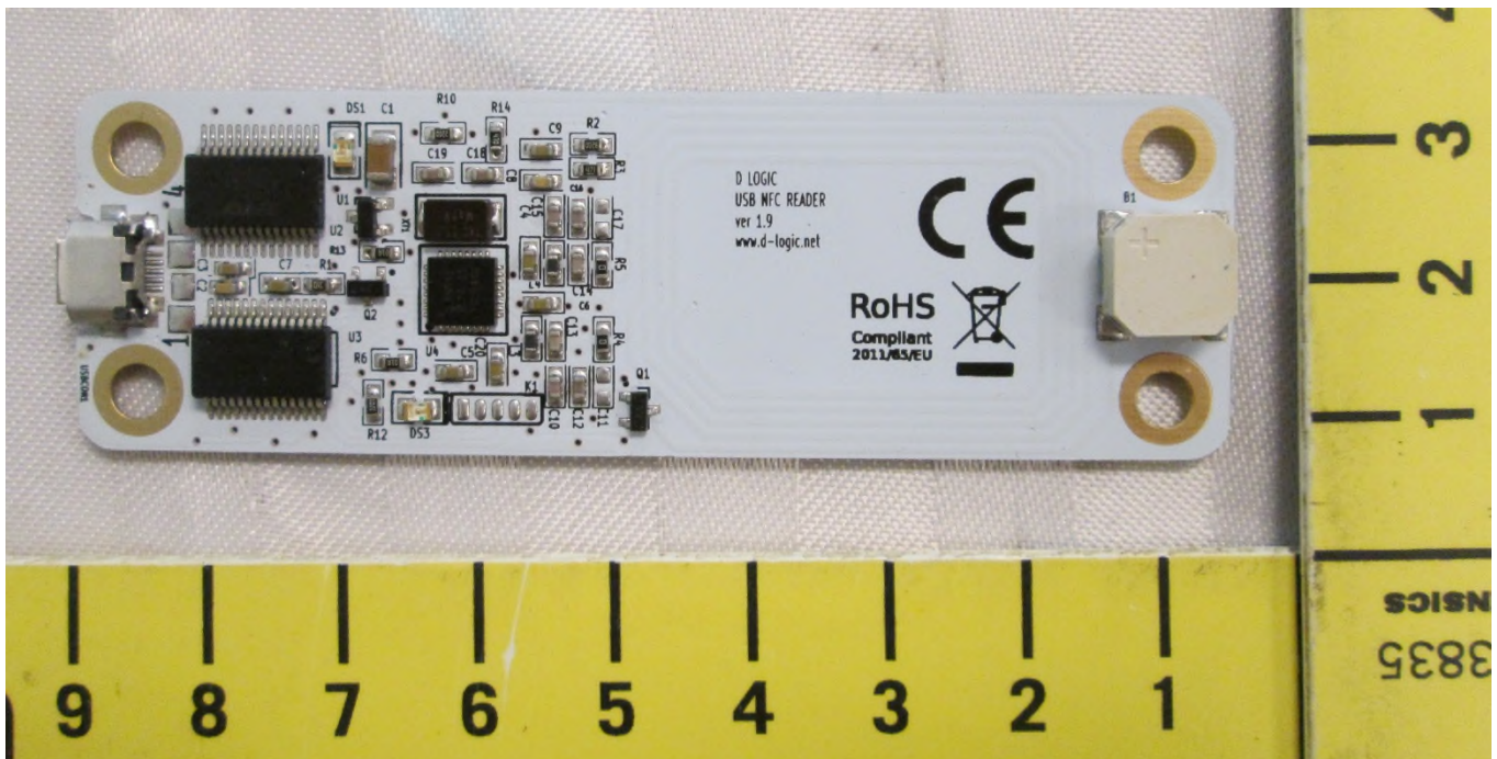
EUT – Internal view 11 NFC board, side 2
