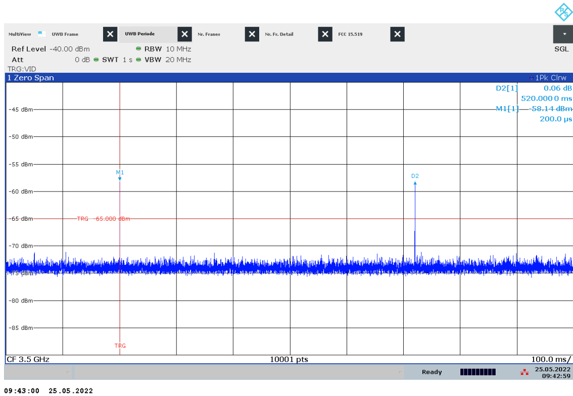
Plot 26: Emission of EUT without associated receiver (for comparison), normal mode, Channel 1
