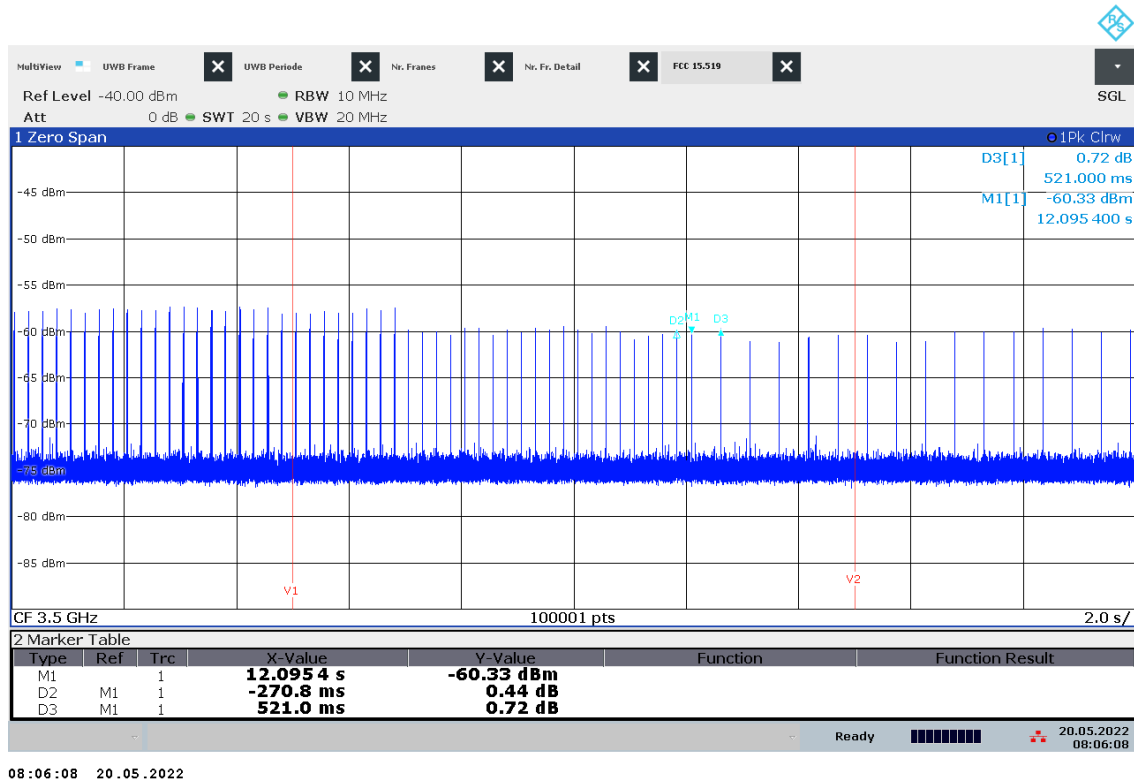
Plot 25: Emissions of the EUT, only at the beginning with associated receiver (Normal mode), Channel 1
