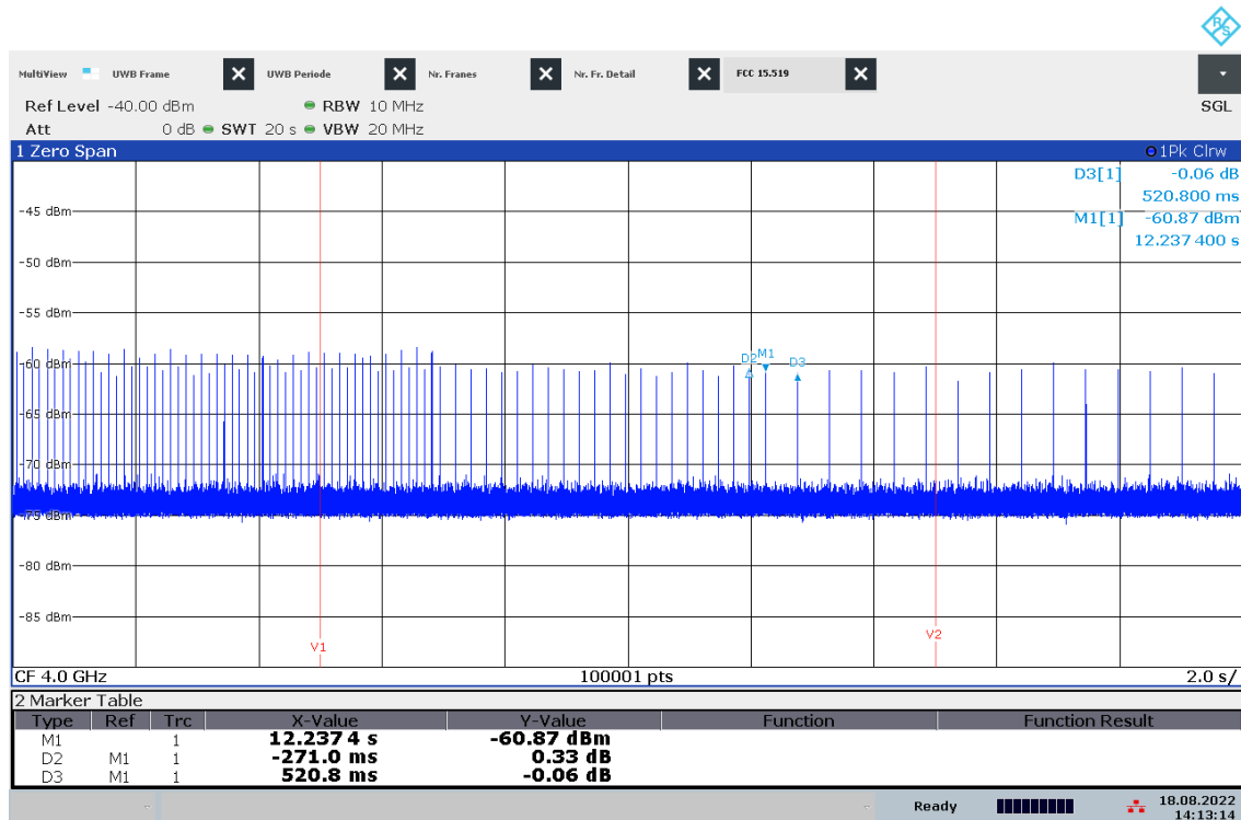
Plot 27: Emissions of the EUT, only at the beginning with associated receiver (Normal mode), Channel 1
